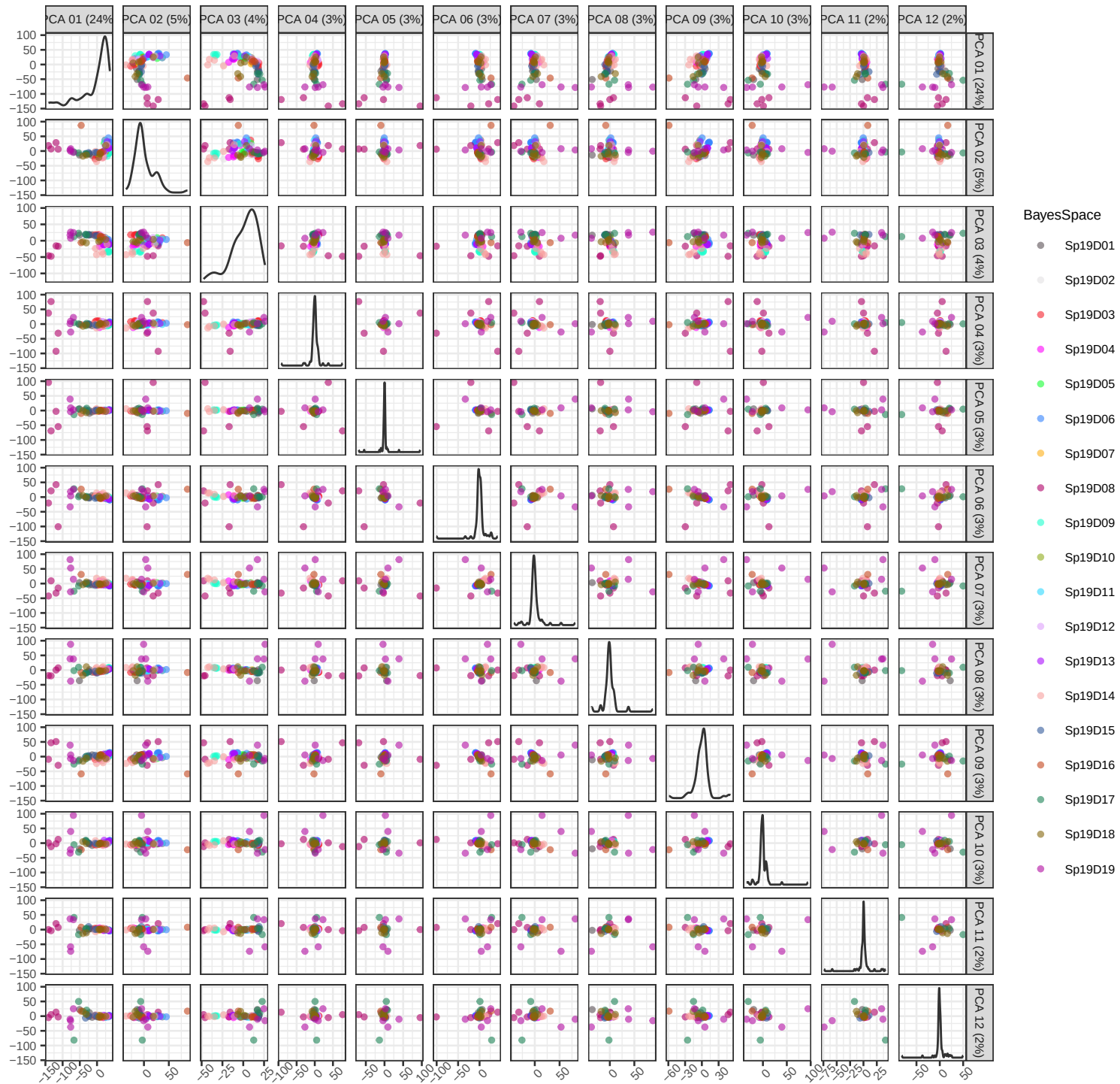
PCA of pseudobulk data with BS k=19
