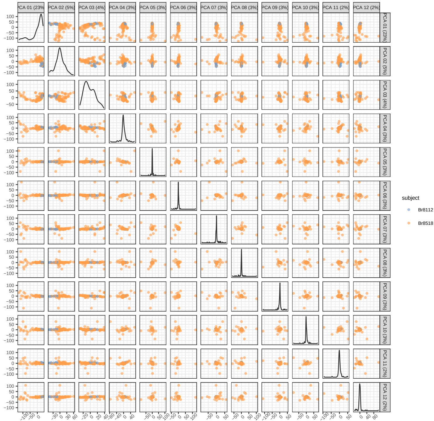
PCA of pseudobulk data with BS k=21
