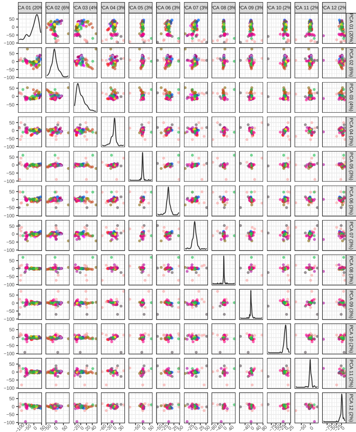
PCA of pseudobulk data with BS k=22
