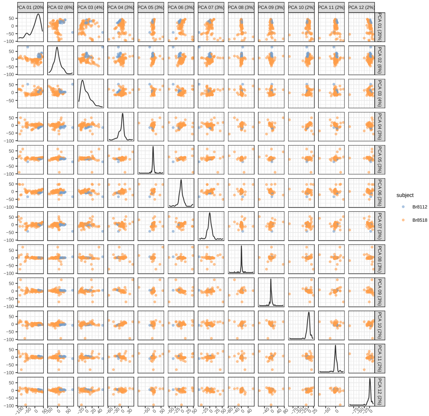
PCA of pseudobulk data with BS k=22
