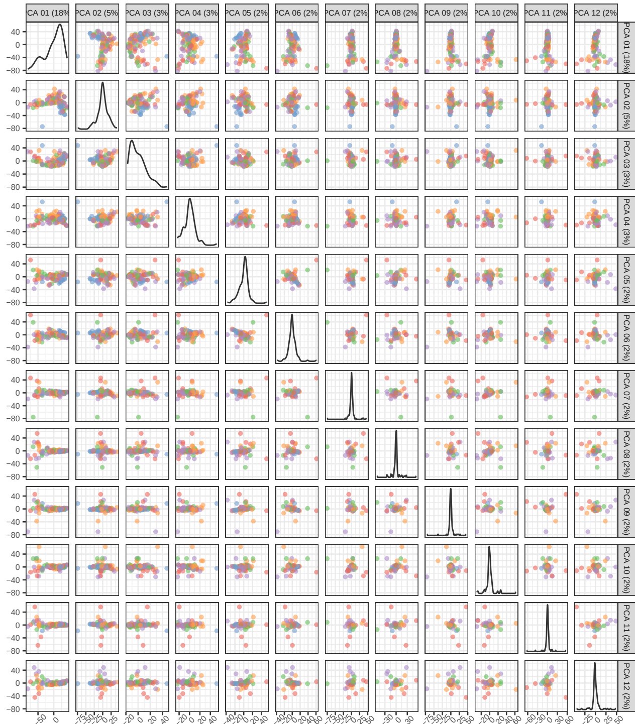
PCA of pseudobulk data with BS k=26
