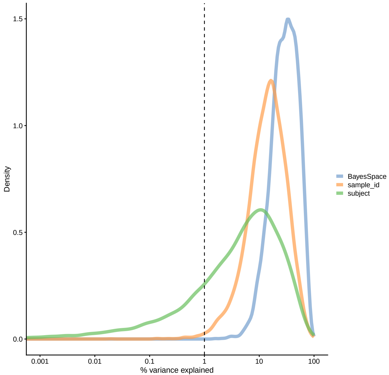
PCA of pseudobulk data with BS k=8
