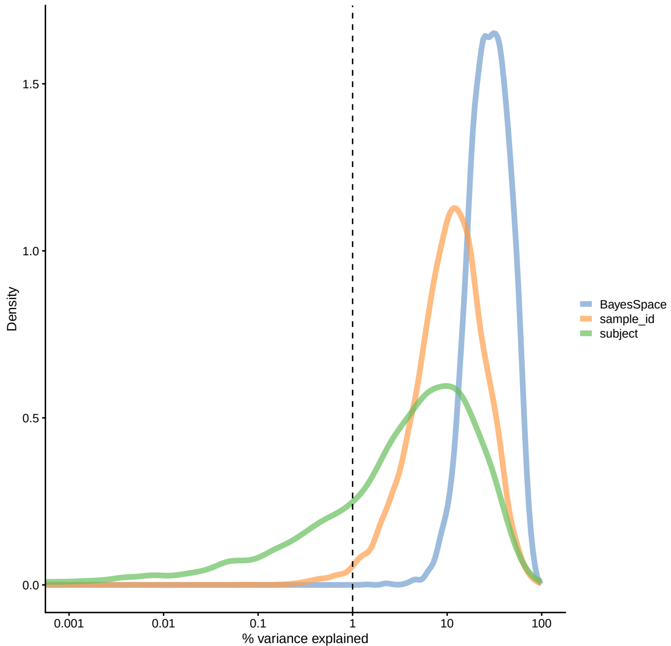
PCA of pseudobulk data with BS k=10
