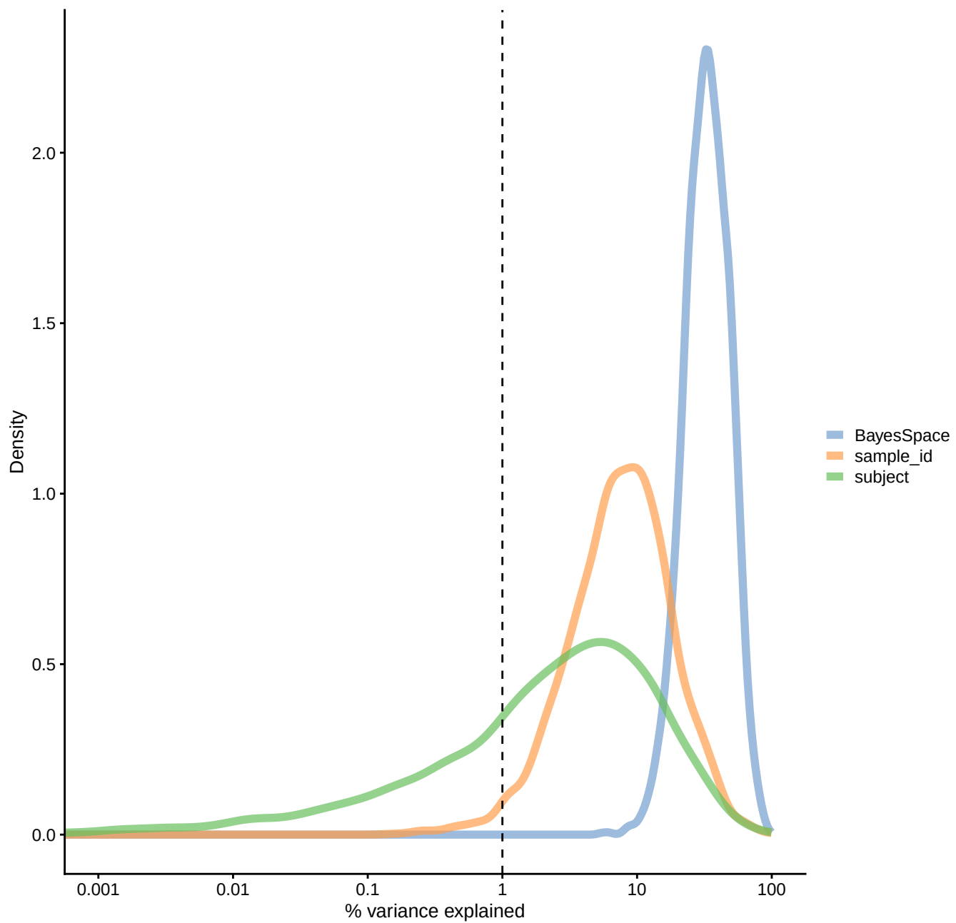
PCA of pseudobulk data with BS k=16
