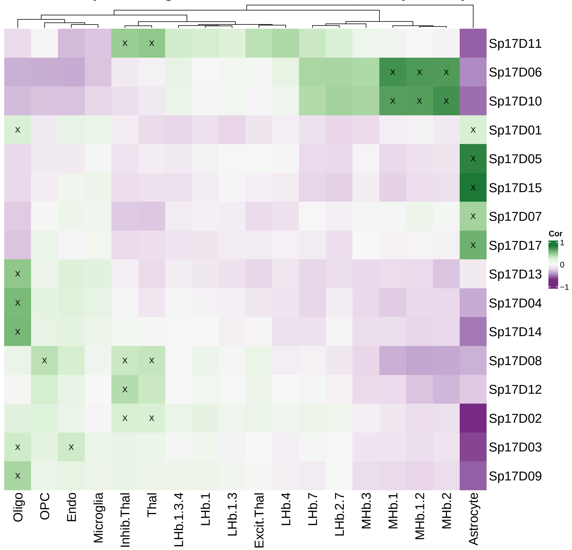
Spatial-Registration: Visium vs Multiome (mid res)
