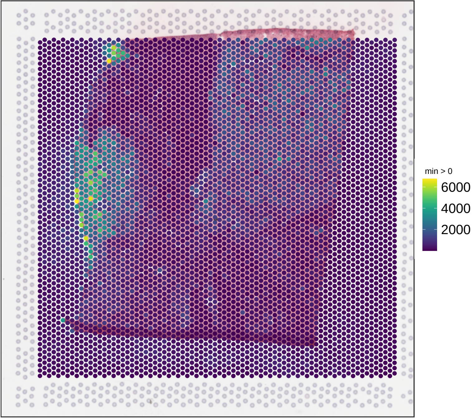
V13B23-285_D1 sum_gene
