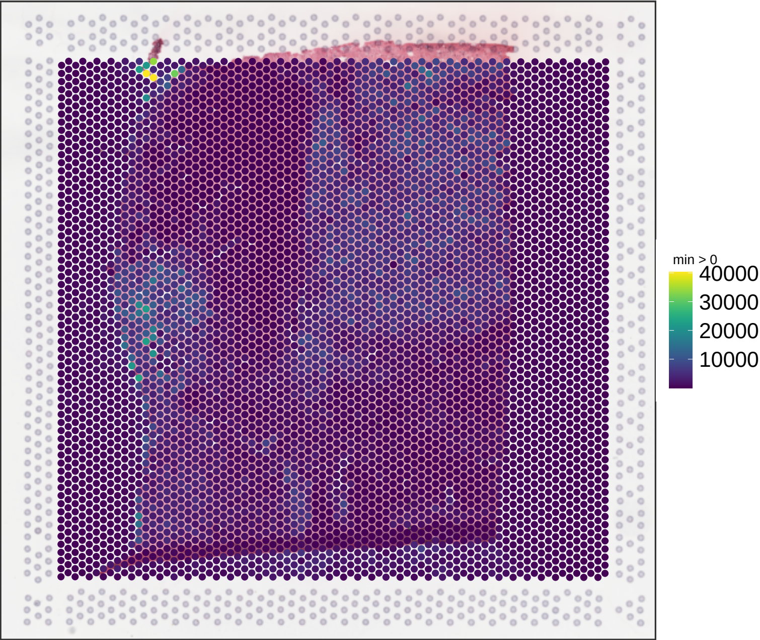
V13B23-285_C1 sum_umi
