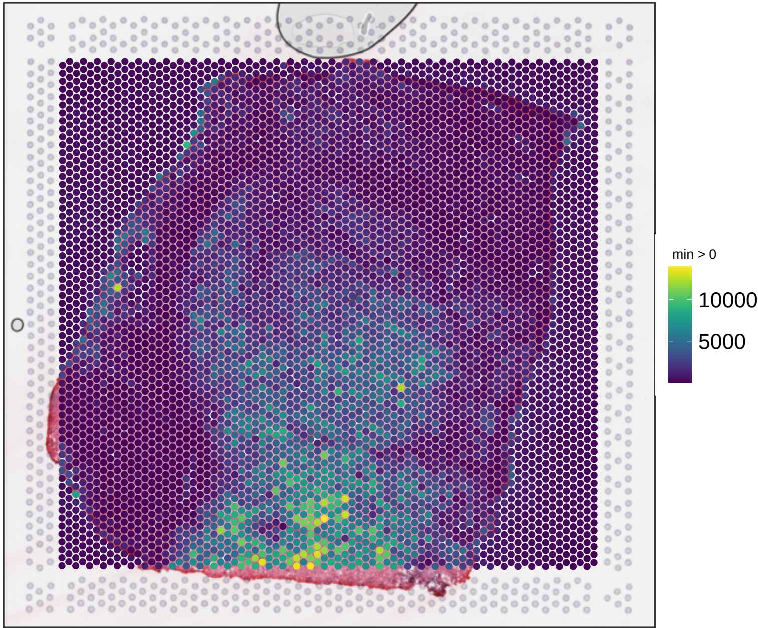
V13B23-285_A1 sum_umi
