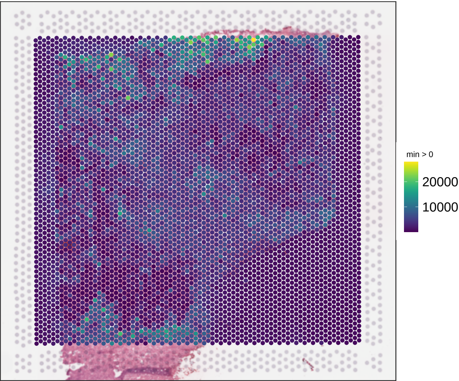
V12D07-075_C1 sum_umi
