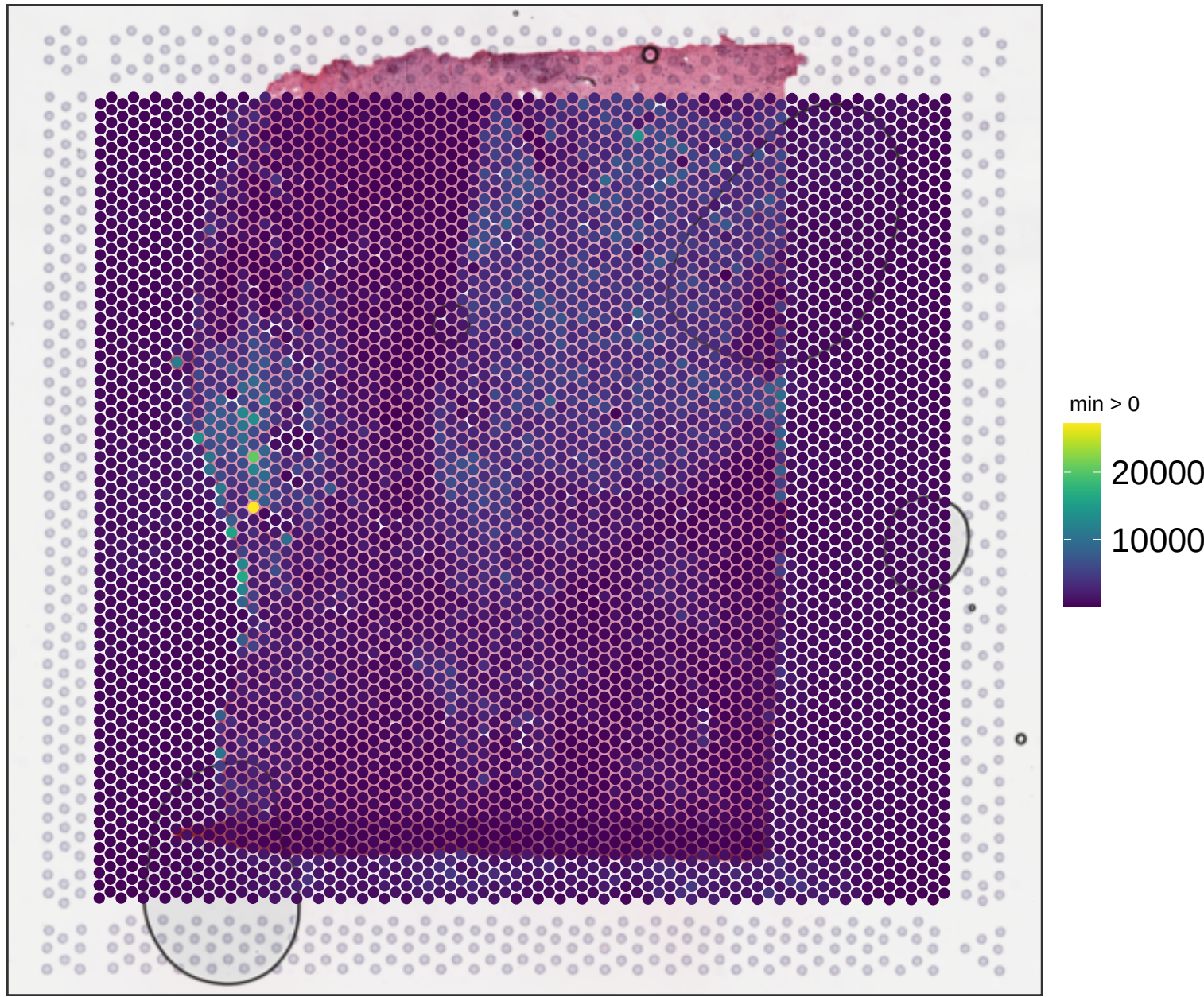
V13B23-285_B1 sum_umi
