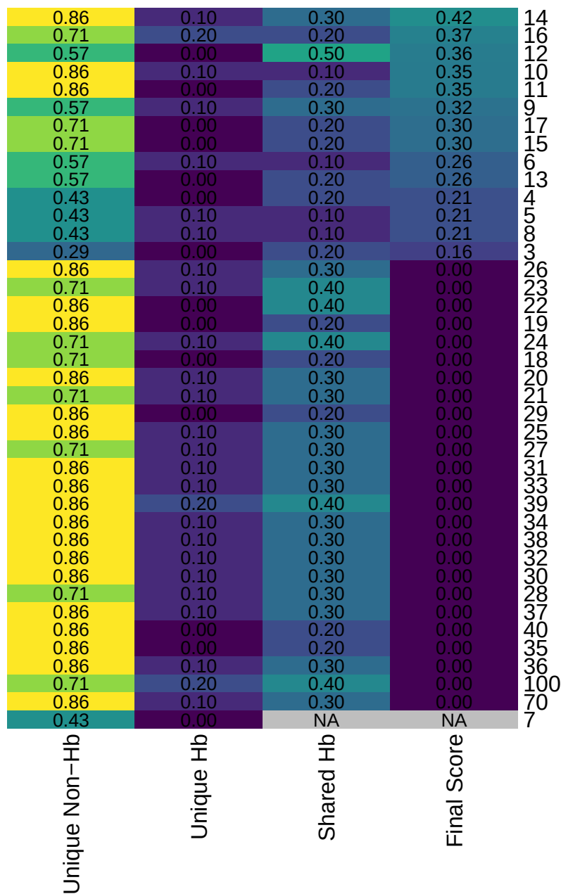
Metric
