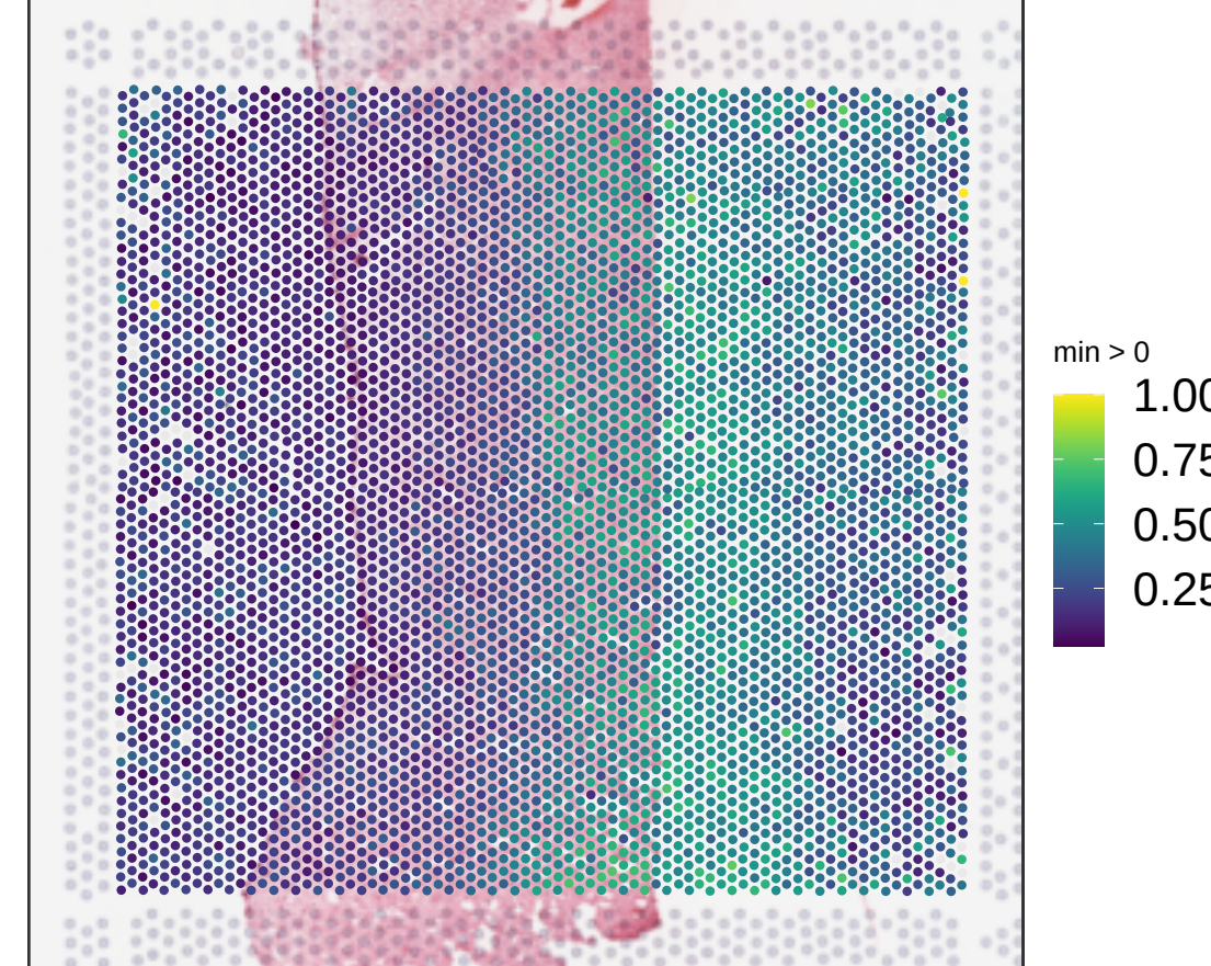
V14F07-340_D1 expr_chrM_ratio
