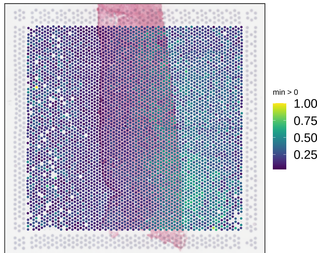
V14F07-340_B1 expr_chrM_ratio
