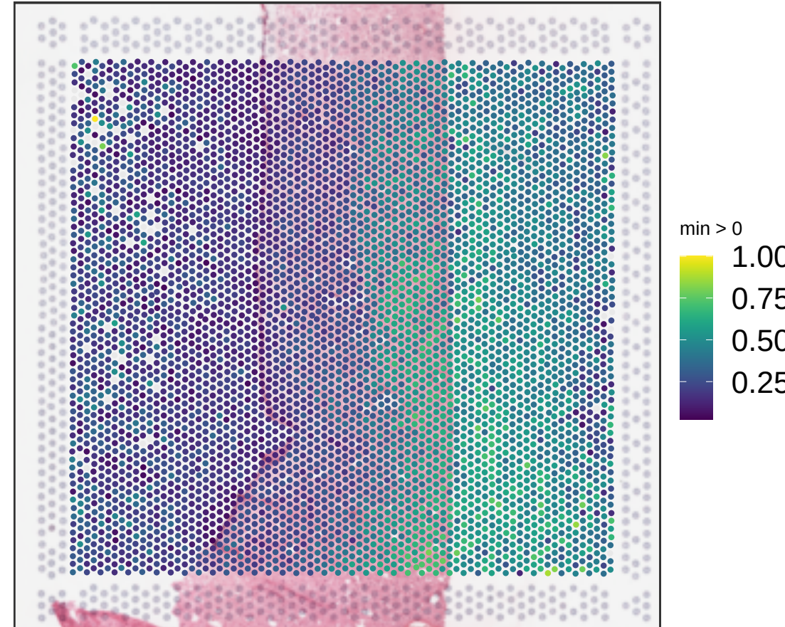
V14F07-340_C1 expr_chrM_ratio
