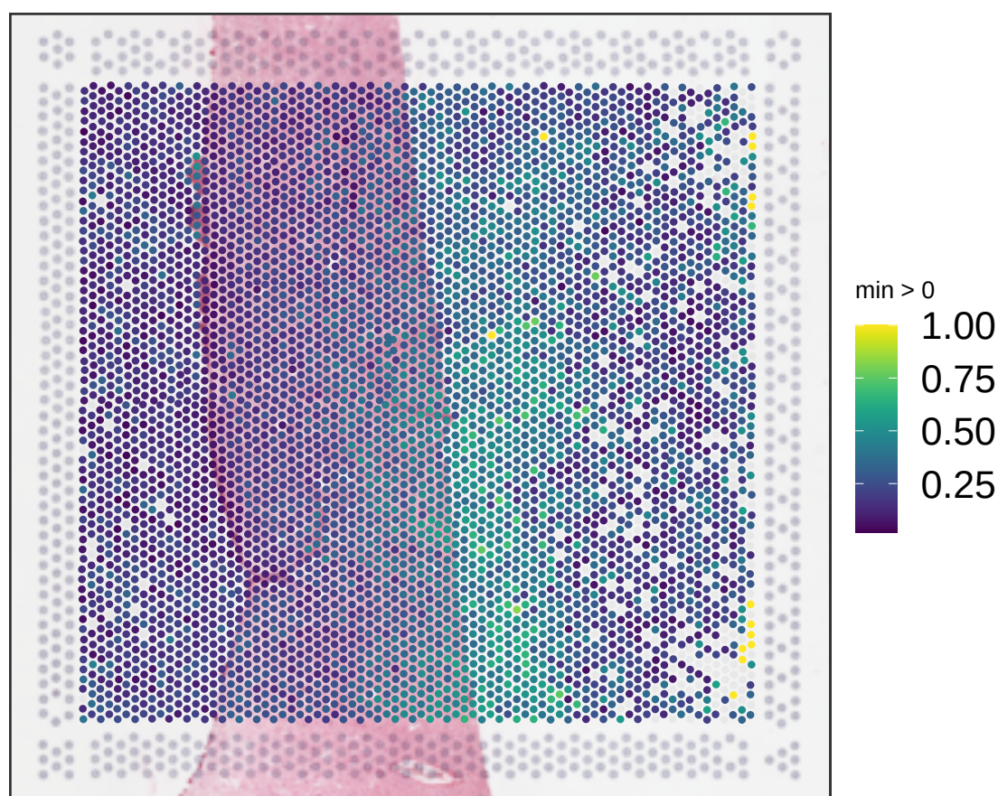
V14F07-340_A1 expr_chrM_ratio
