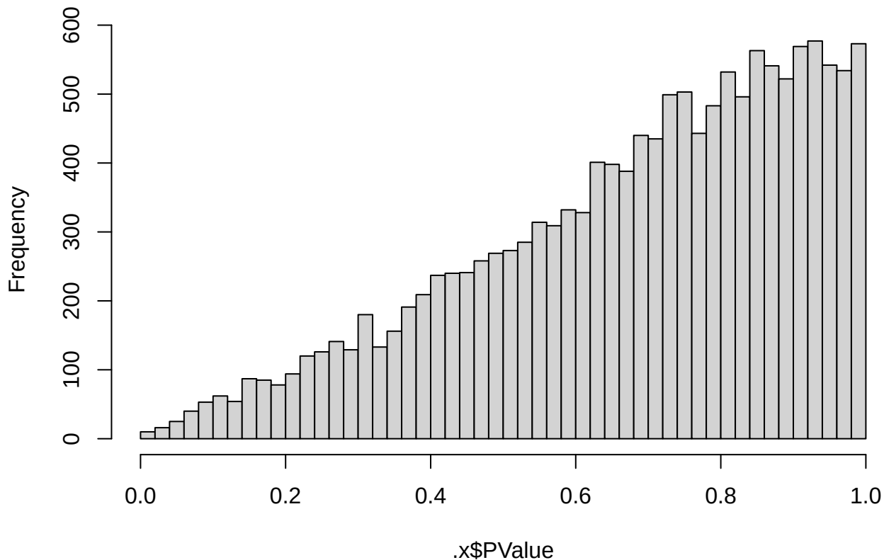
Histogram of raw p-values
