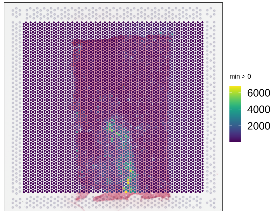
V13B23-281_B1 sum_umi
