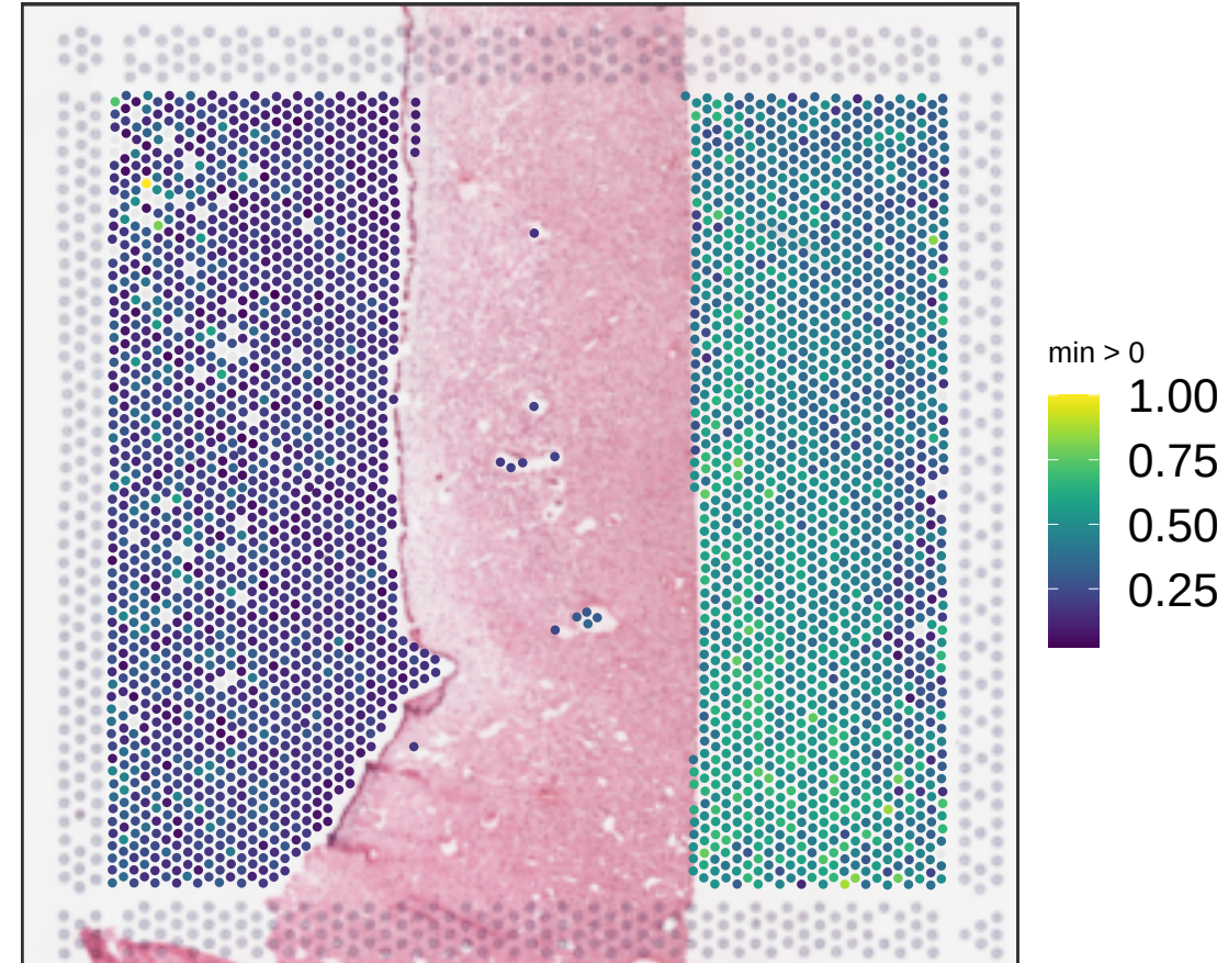
V14F07-340_C1 expr_chrM_ratio
