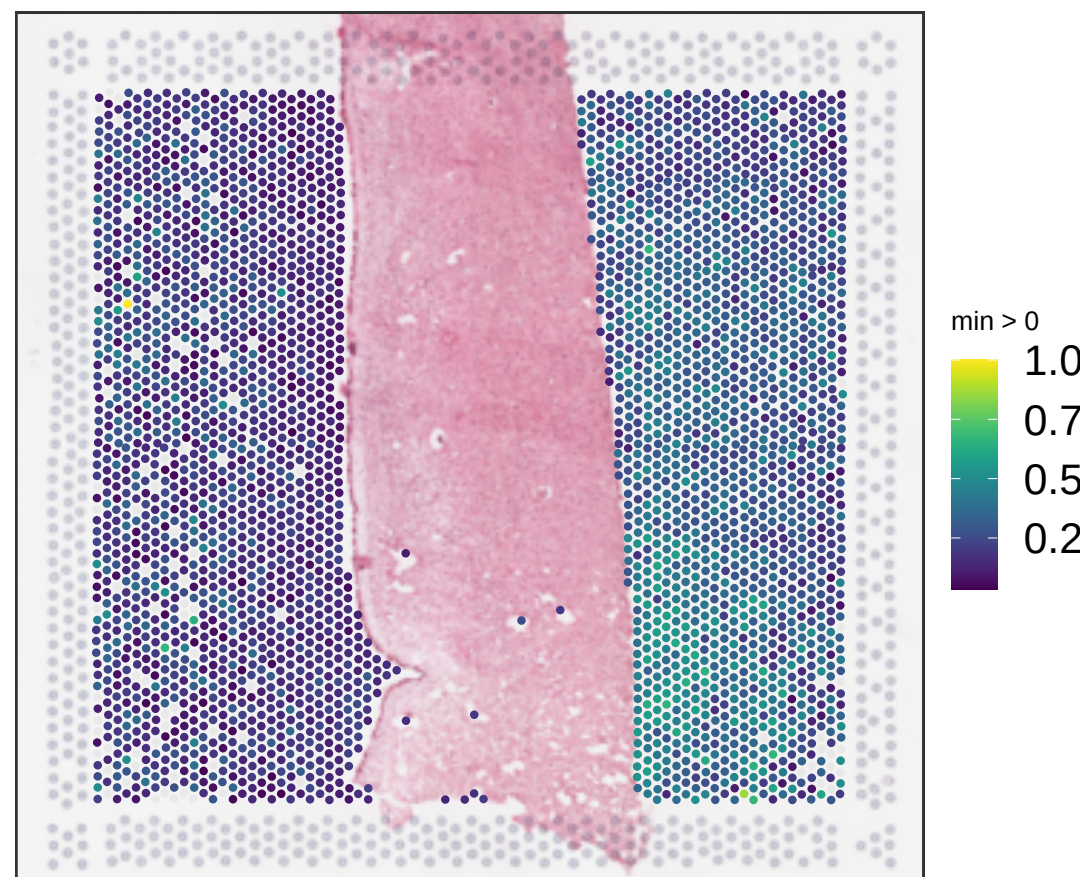
V14F07-340_B1 expr_chrM_ratio
