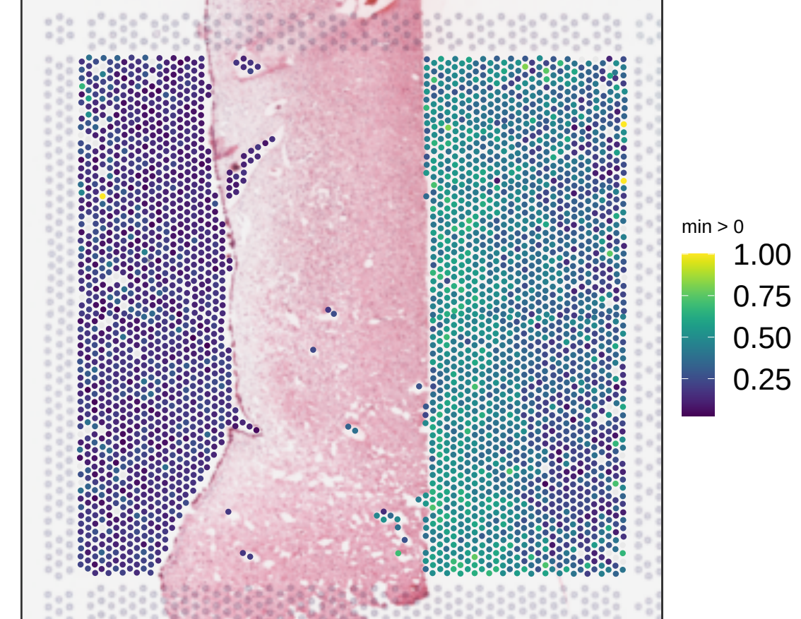
V14F07-340_D1 expr_chrM_ratio
