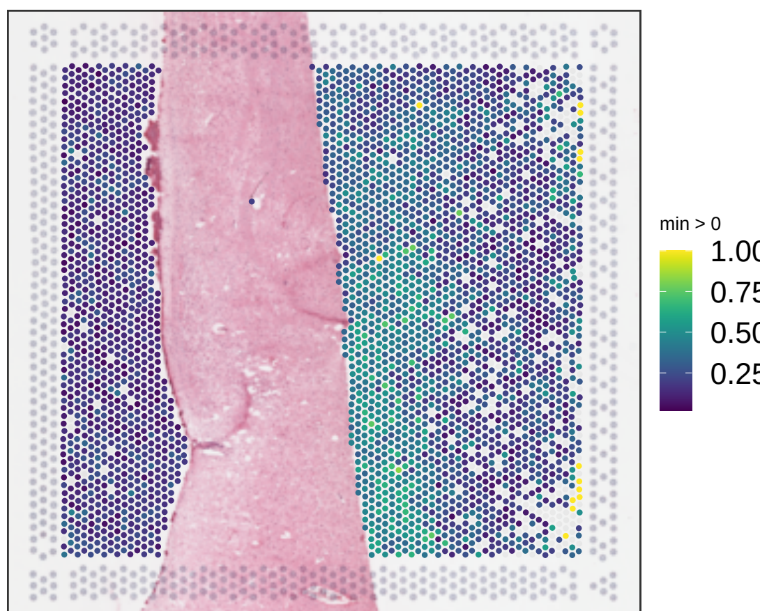
V14F07-340_A1 expr_chrM_ratio
