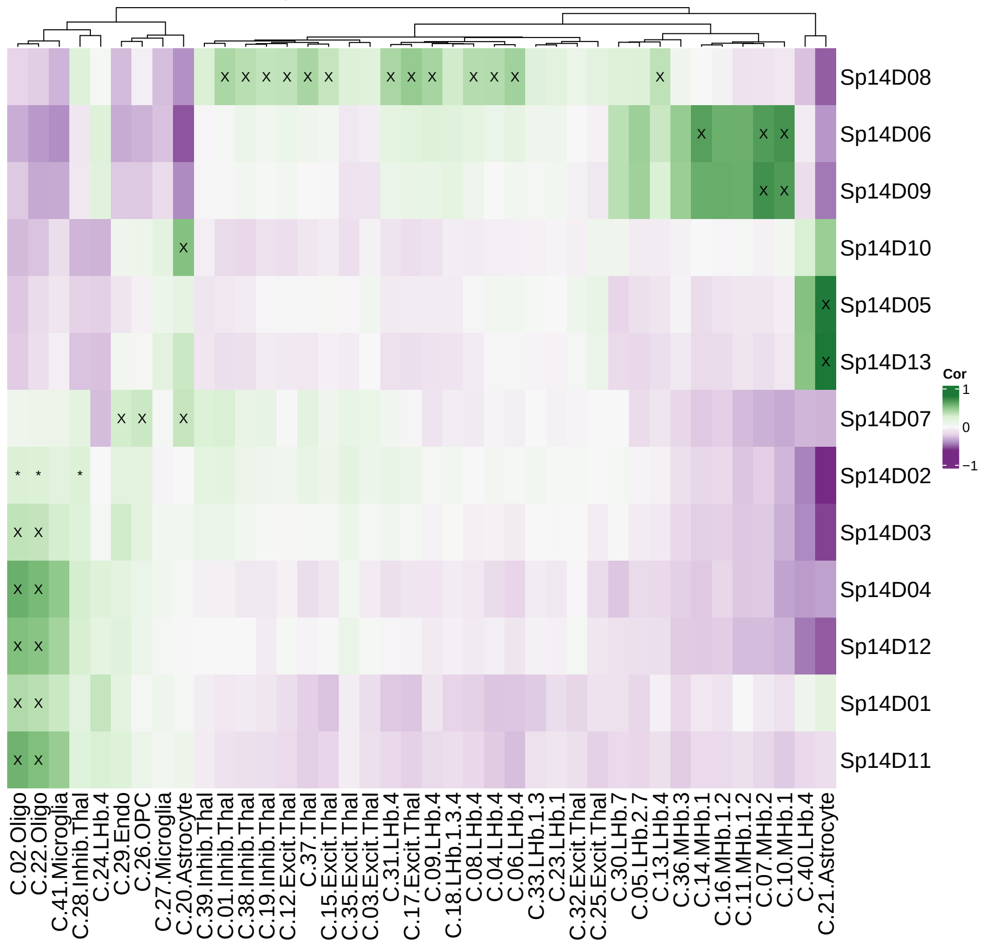
Spatial-Registration: Visium vs Multiome (Fine res)
