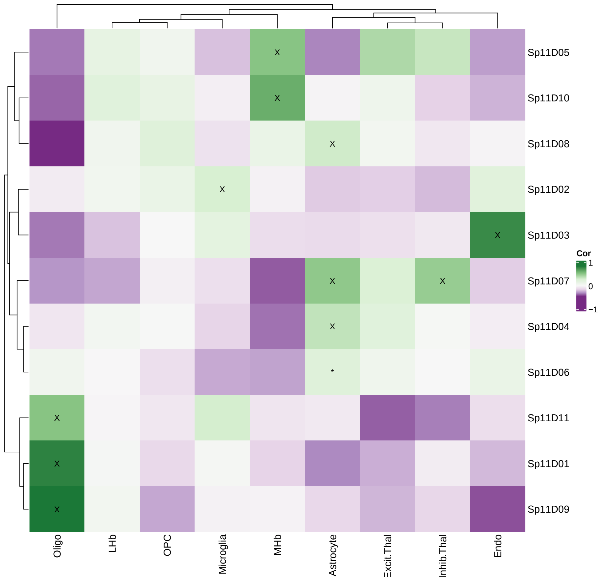
Spatial-Registration: Visium vs snRNA (Broad res)
