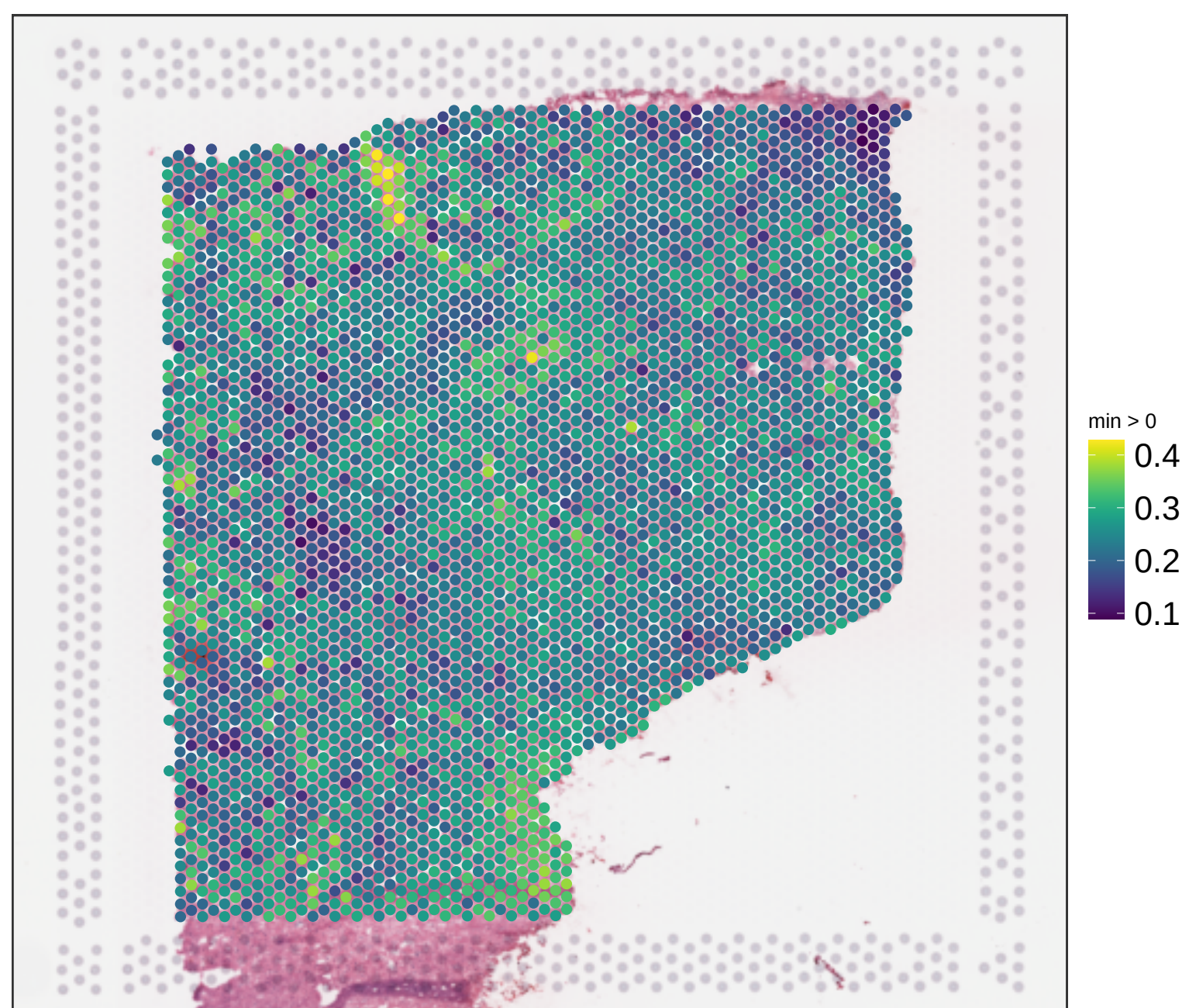
V12D07-075_C1 expr_chrM_ratio
