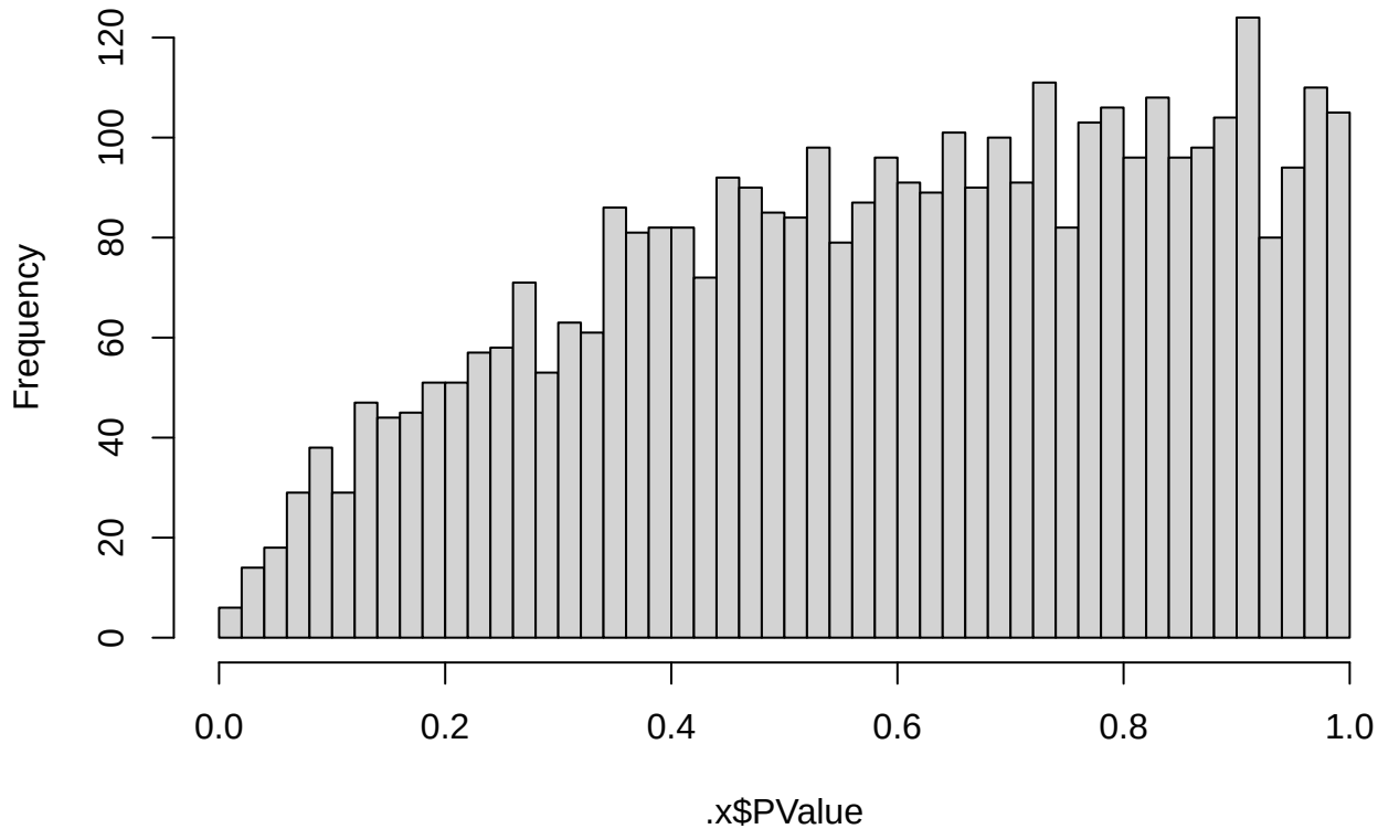
Histogram of raw p-values
