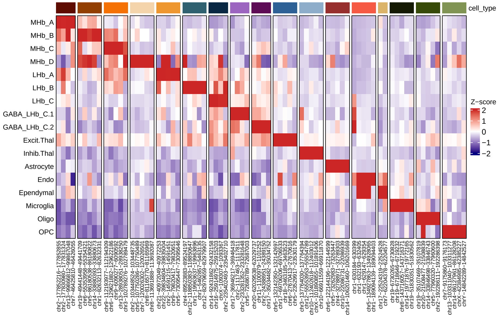
Top DAR Peaks per Cell Type
