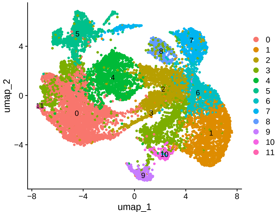
integrated_snn_res.0.3
