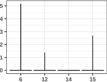
MMRN1
