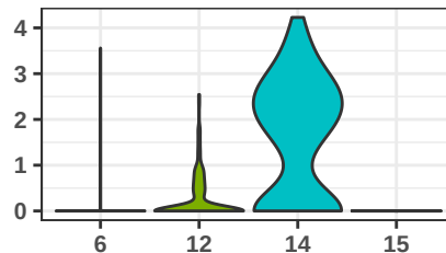
RASGRP1
