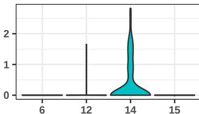
LINC02143
