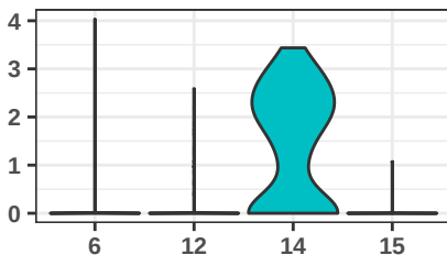
SLC5A7
