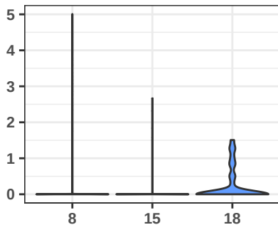
MMRN1
