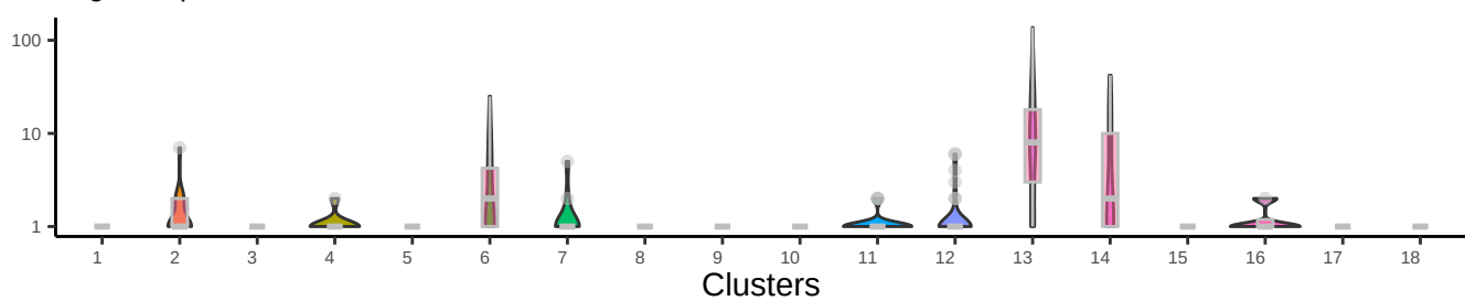
Log10 Exp – MMRN1
