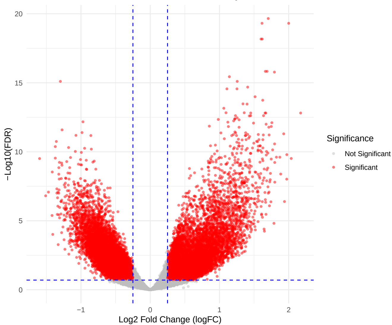
Volcano Plot for DARs in Astrocyte
