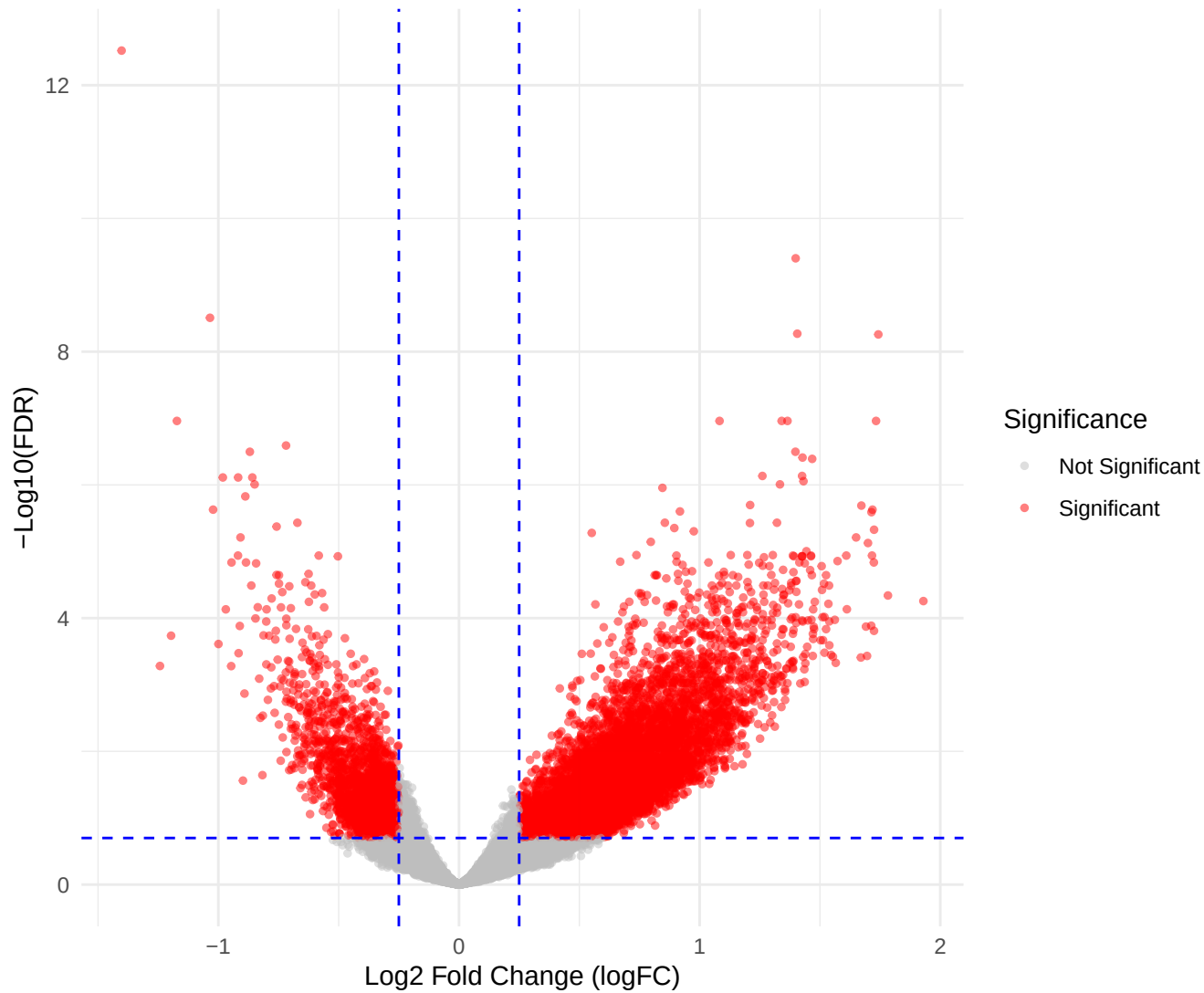
Volcano Plot for DARs in LHb.1
