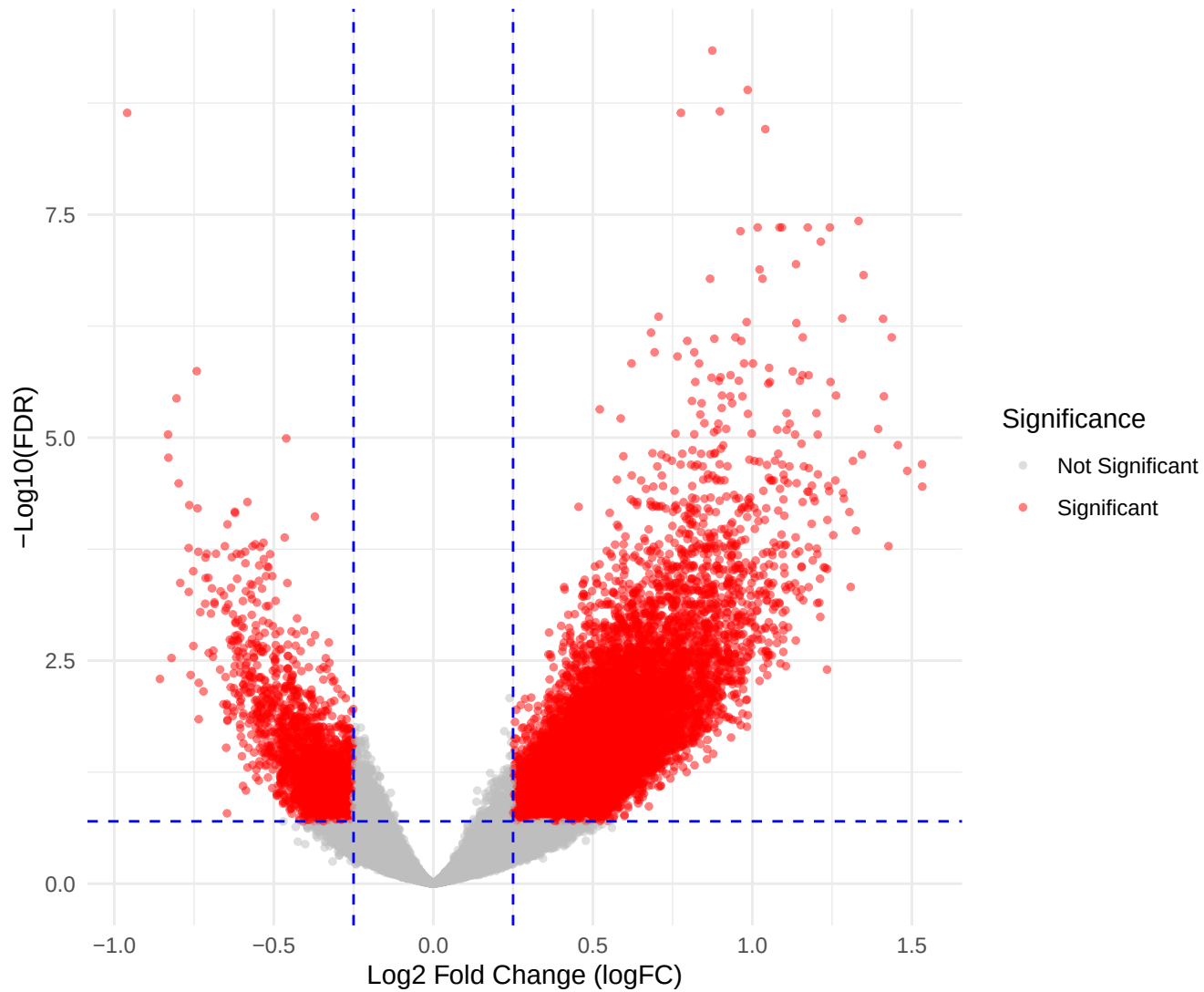
Volcano Plot for DARs in LHb.2.7
