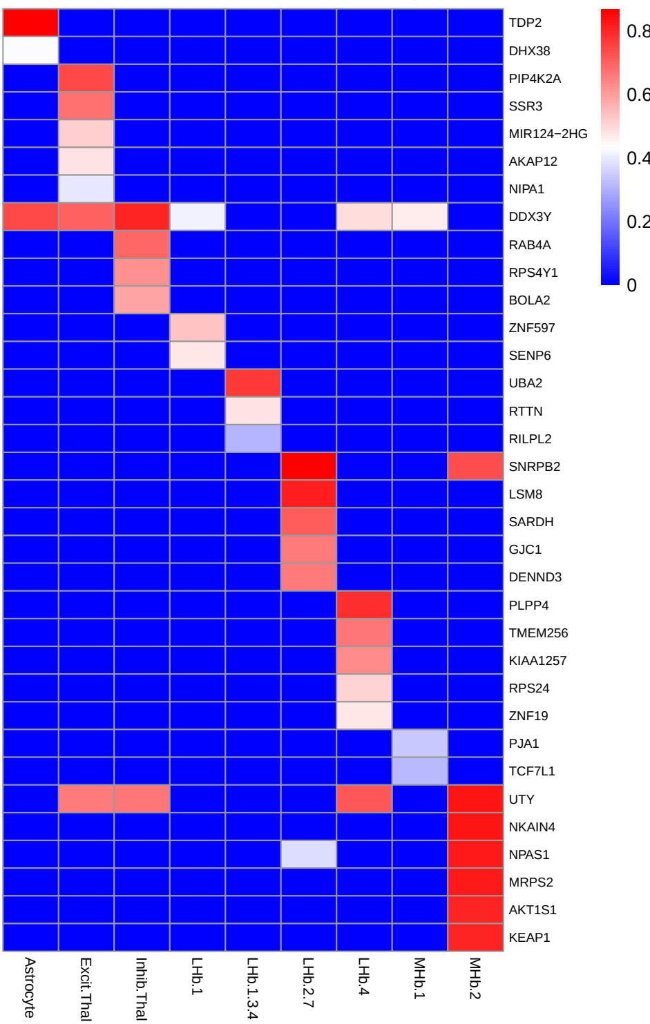
Linked DAR enriched/nPlotted 34 peaks
