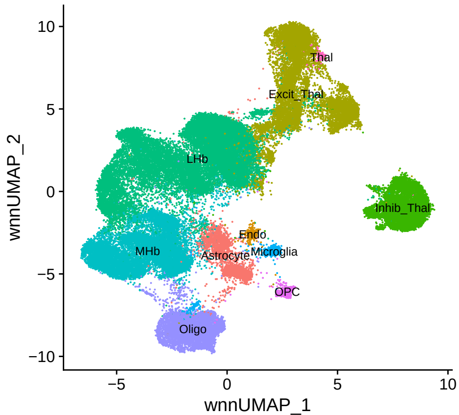
**WNN Merged Clusters
