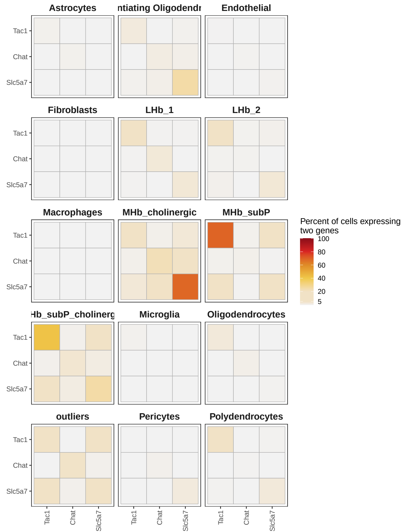
Co-expression of SubP and Chol markers in Wallace mouse dataset
