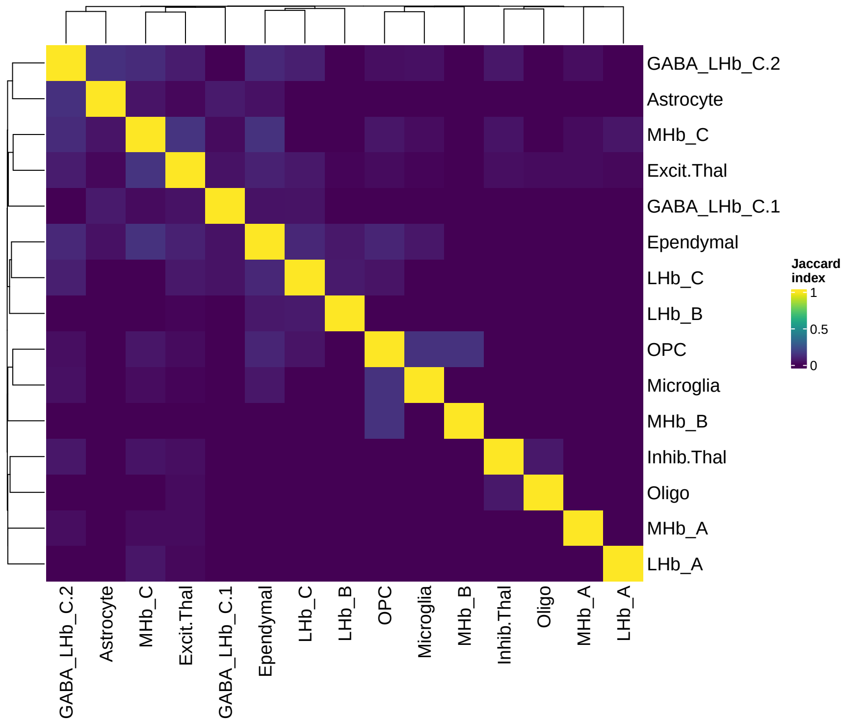
TF set Jaccard index between cell types
