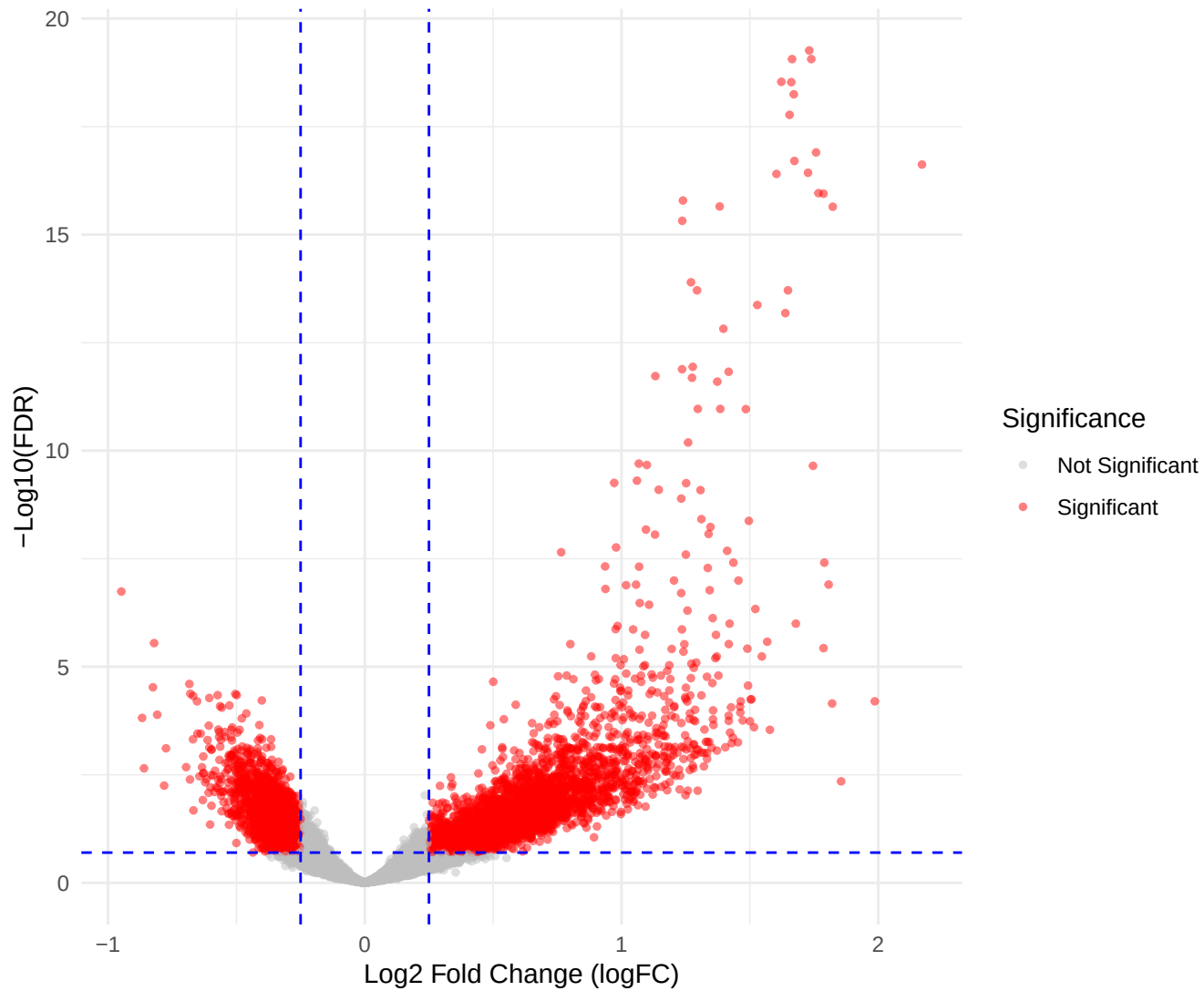
Volcano Plot for DARs in MHb.1.2
