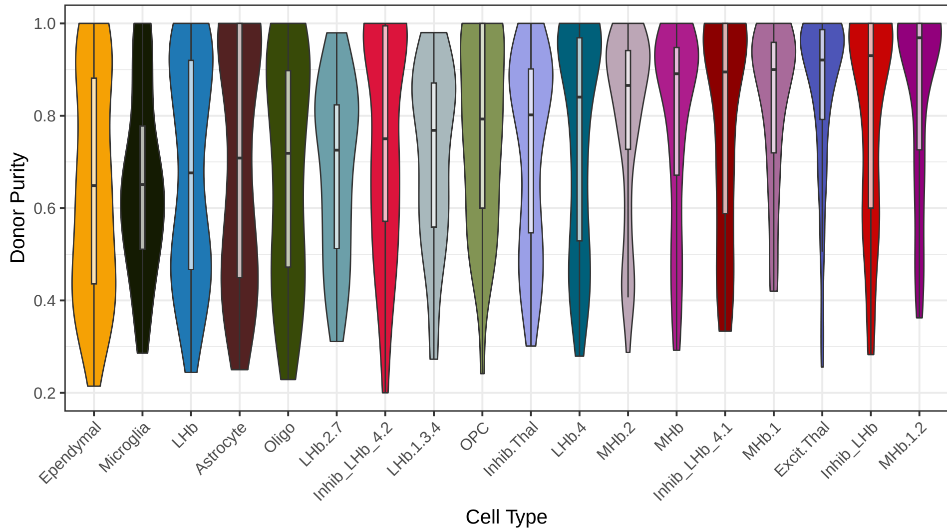
Donor Purity by Cell Type
