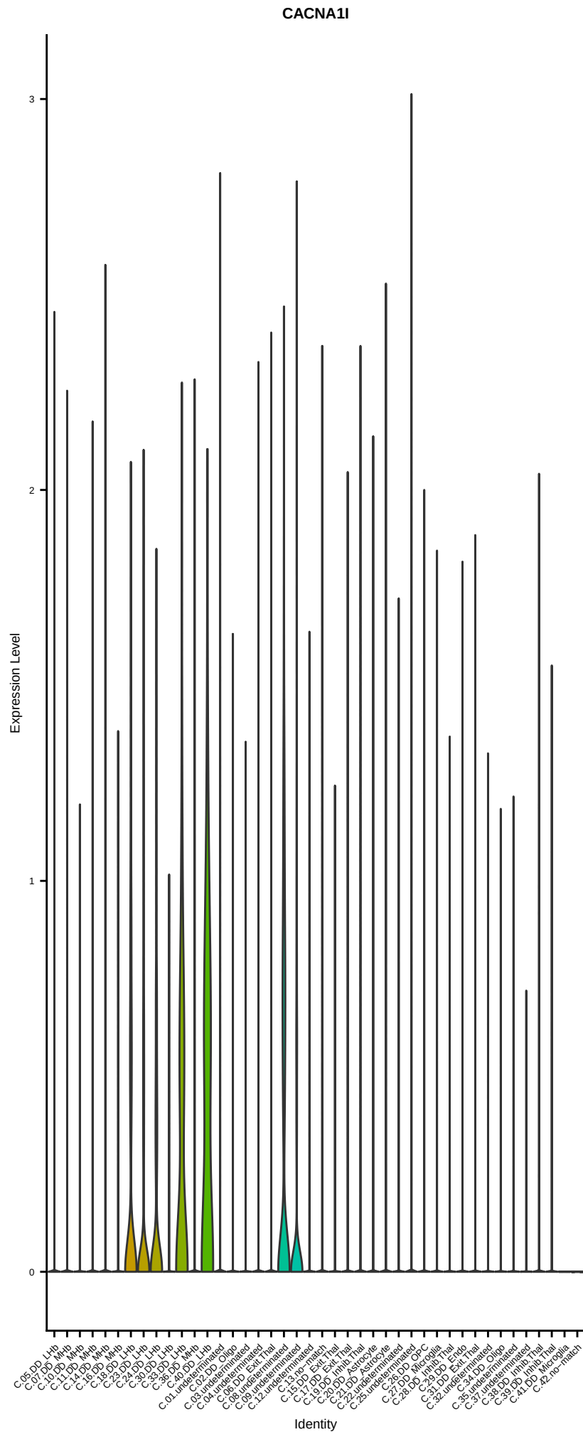
Top 10 genes in cluster: 40
