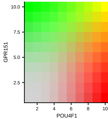
**Clusters from WNN: C.SLM_Isi_r1
