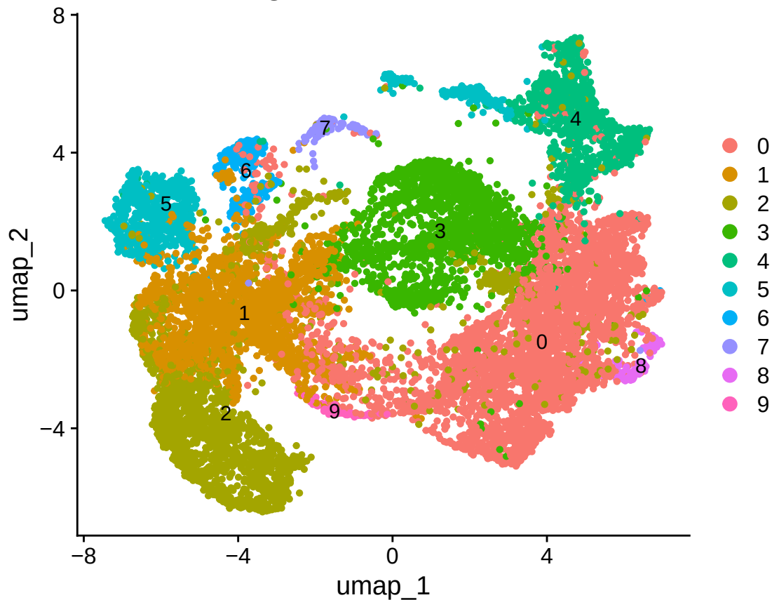
integrated_snn_res.0.25
