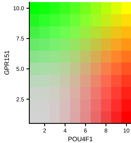
**Clusters from WNN: k40_C.leiden_Isi_r2
