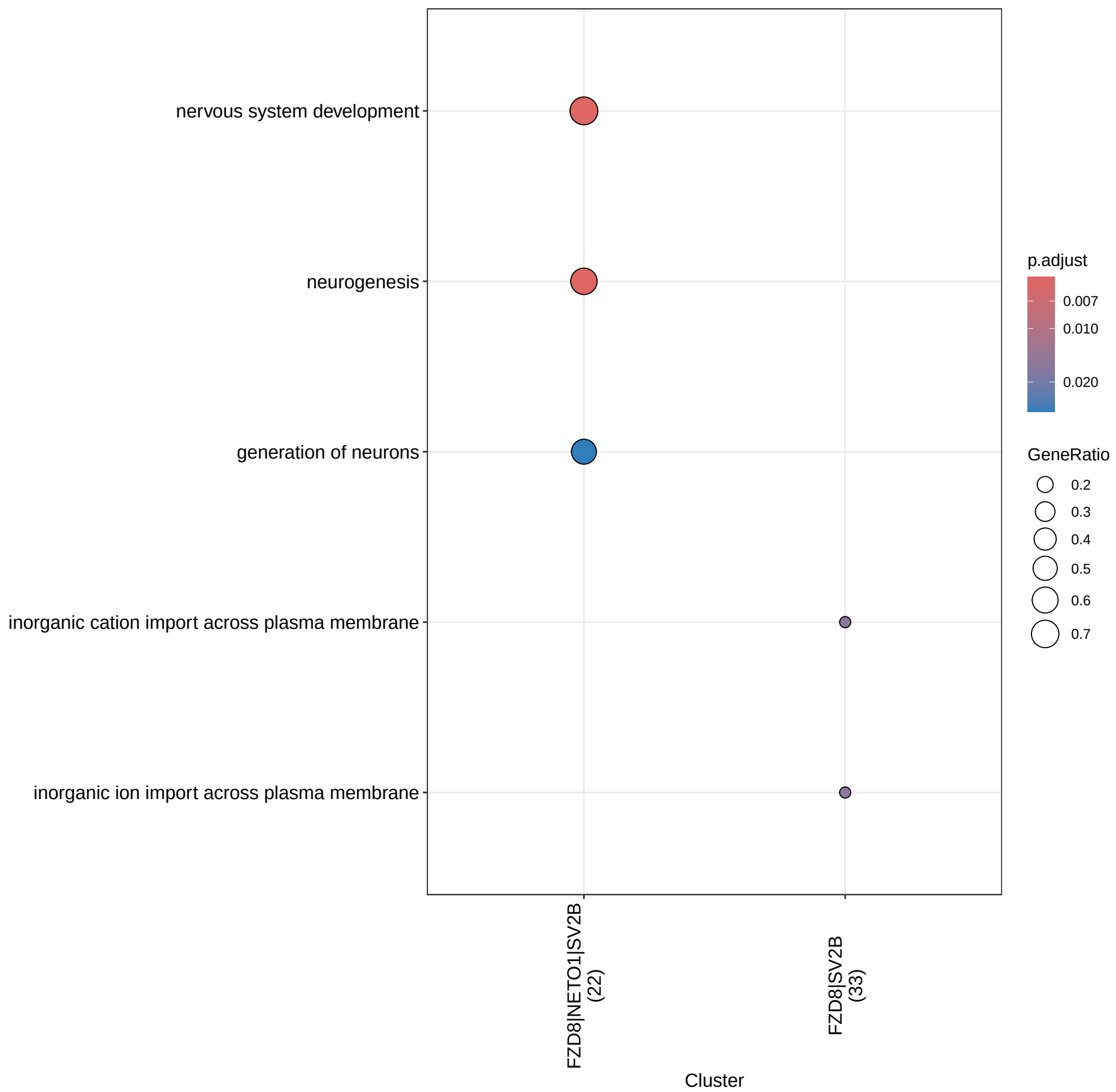
GO Enrichment (mediation groups, 2+ genes): BP
