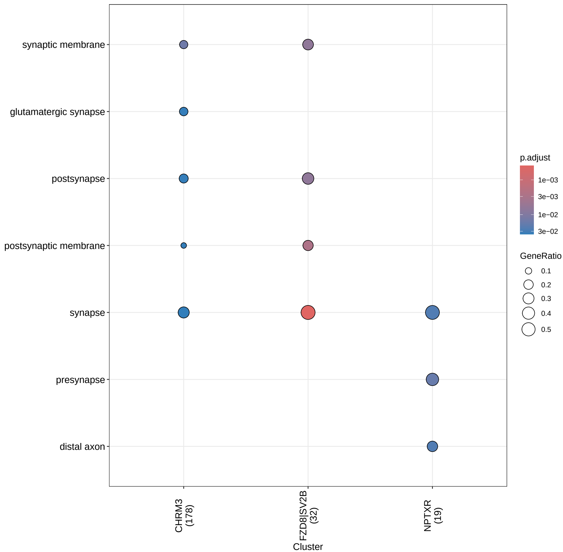
GO Enrichment (mediation groups, 2+ genes): CC
