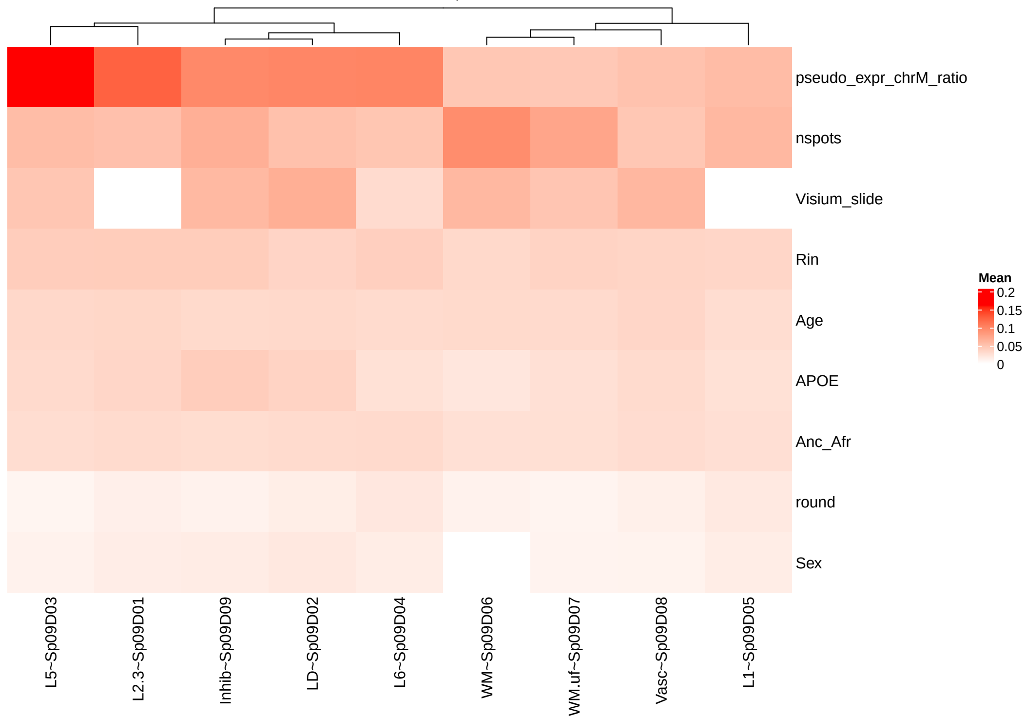
Visium VarPart – apoe
