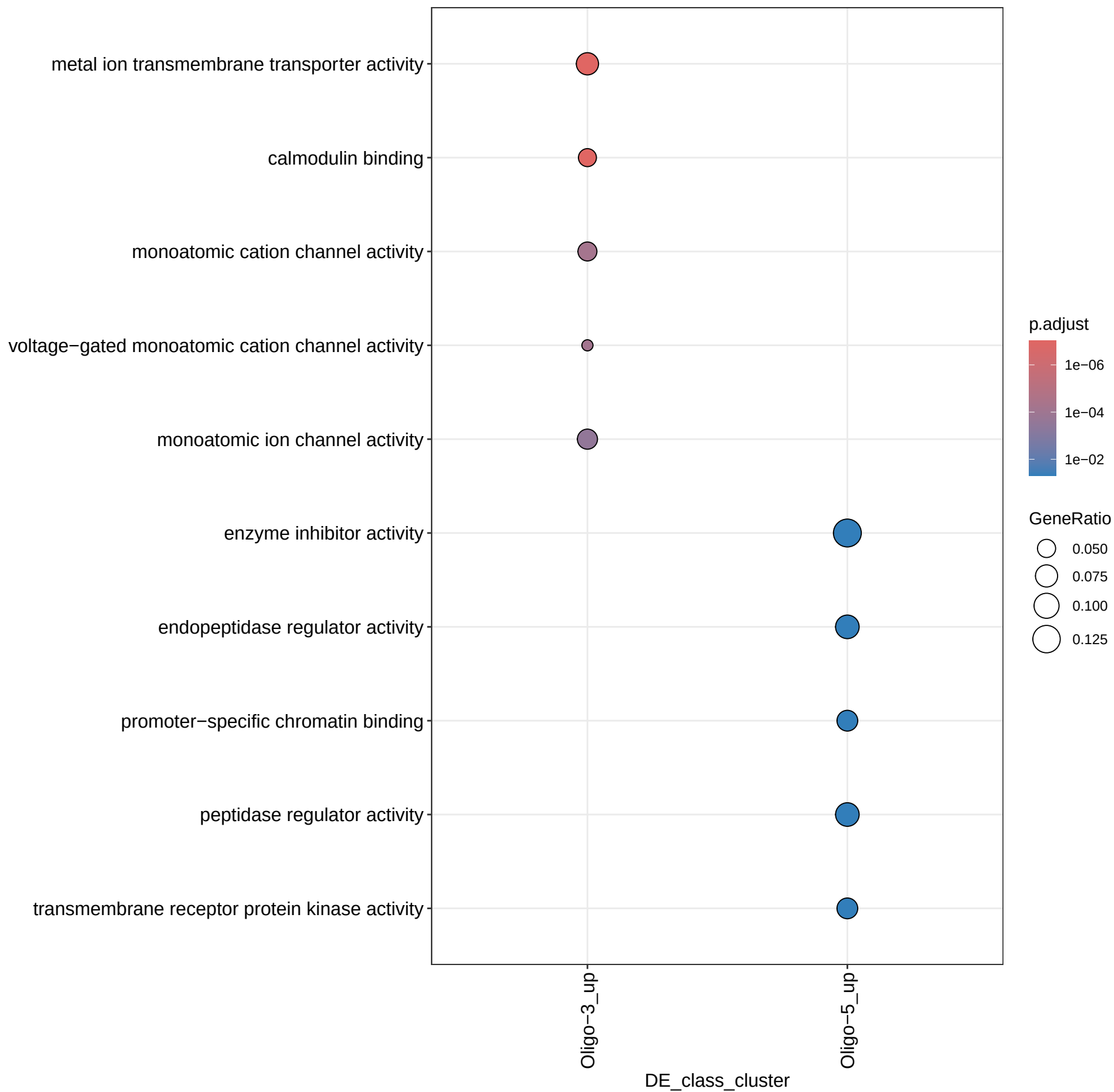
GO Enrichment:MF – Oligo (2+ genes)
