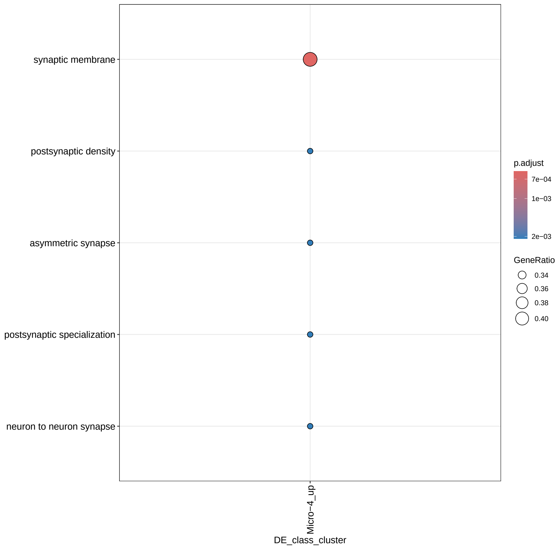
GO Enrichment:CC – Micro (2+ genes)
