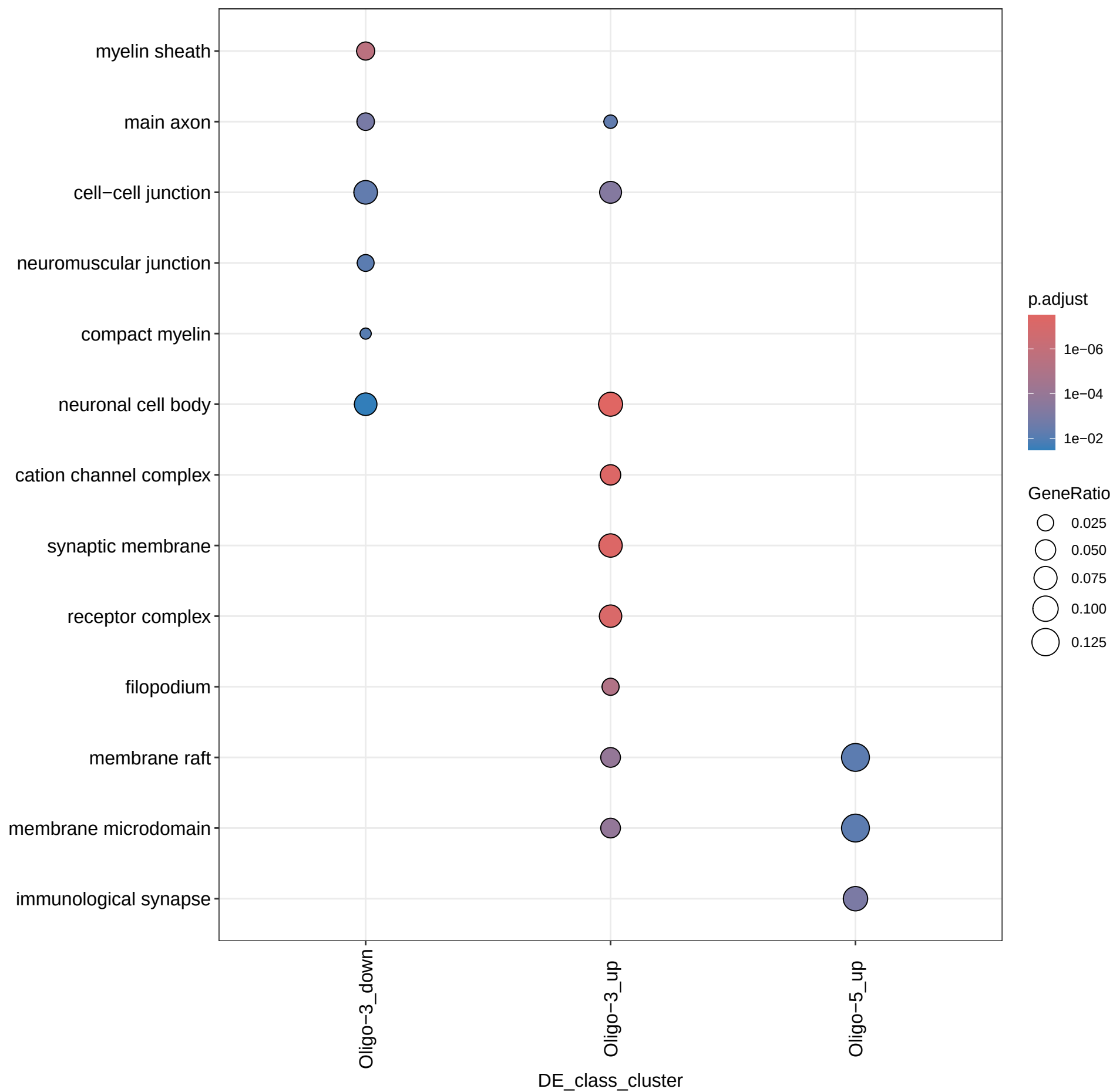
GO Enrichment:CC – Oligo (2+ genes)
