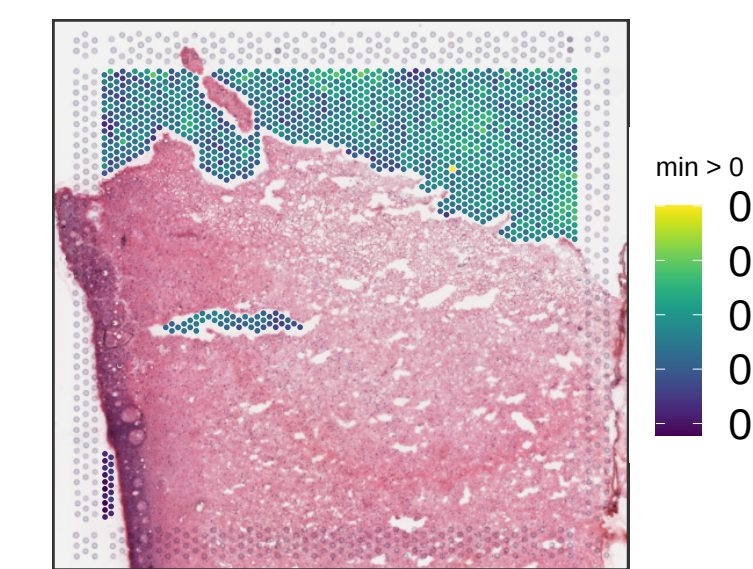
Br1706 expr_chrM_ratio
