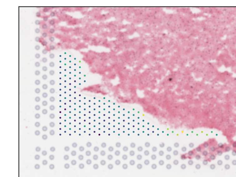
Br5599 expr_chrM_ratio
