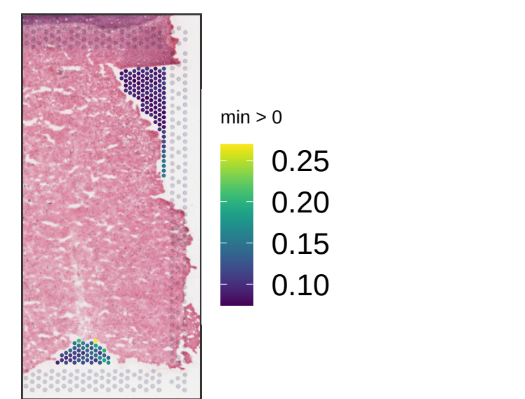
Br5634 expr_chrM_ratio
