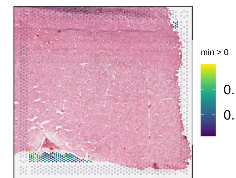
Br5941 expr_chrM_ratio
