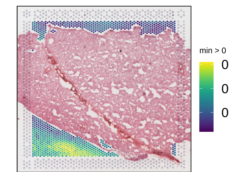
Br1691 expr_chrM_ratio
