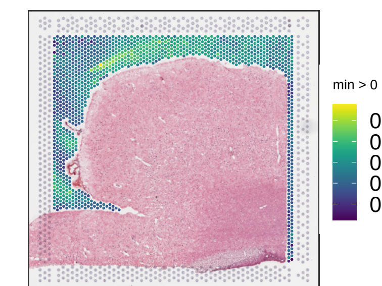
Br5517 expr_chrM_ratio
