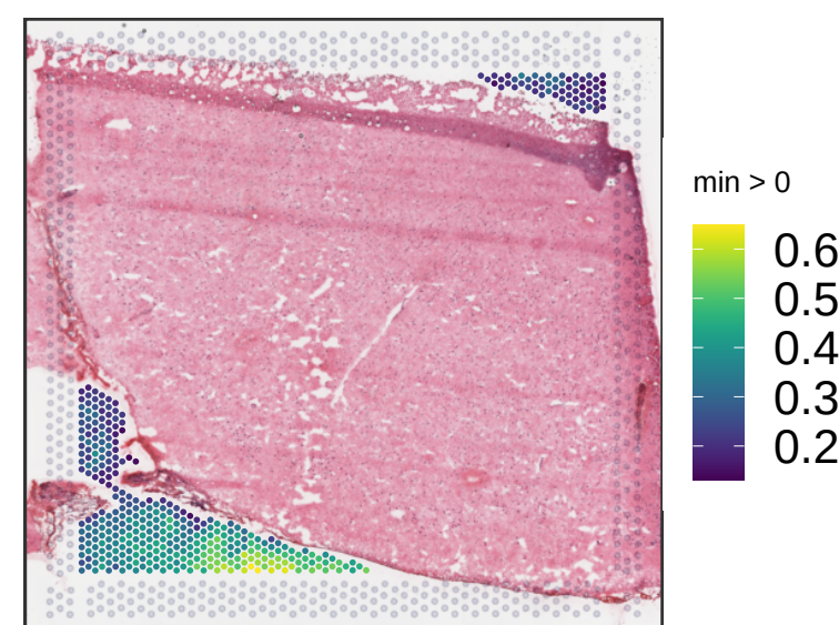
Br6098 expr_chrM_ratio
