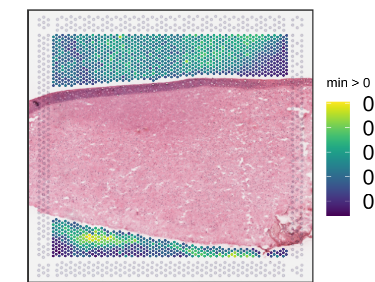
Br5854 expr_chrM_ratio
