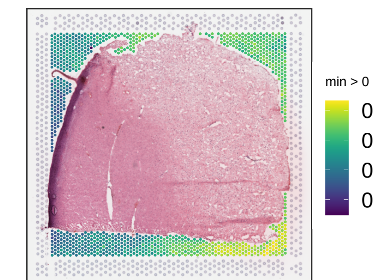
Br5276 expr_chrM_ratio
