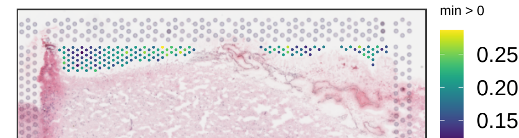
Br5426 expr_chrM_ratio
