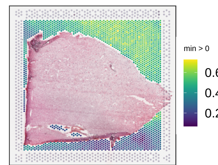
Br5712 expr_chrM_ratio
