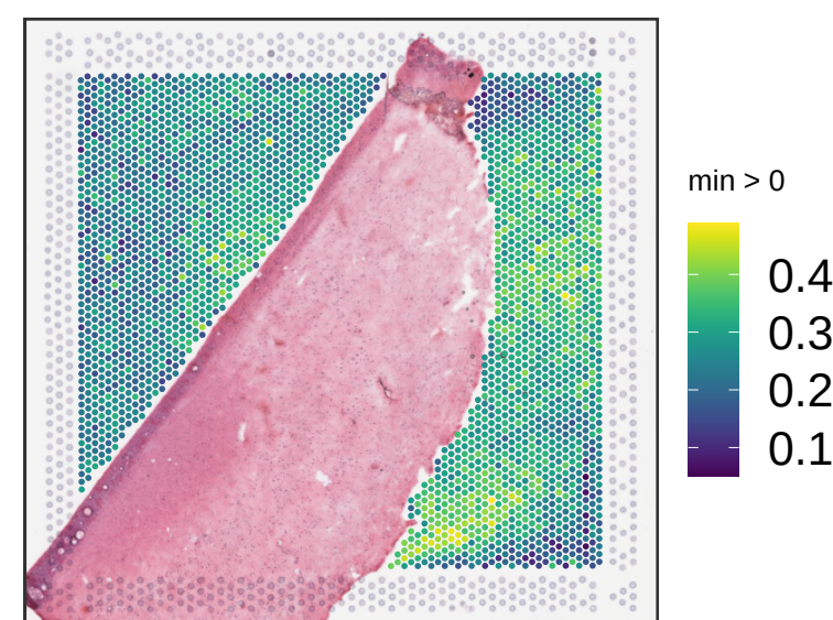
Br2582 expr_chrM_ratio
