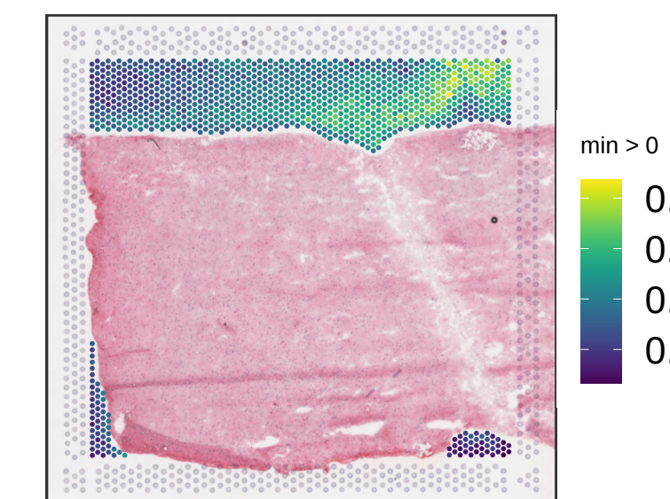
Br6476 expr_chrM_ratio
