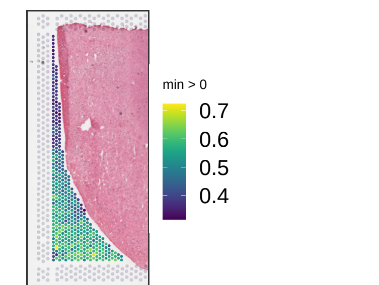
Br5529 expr_chrM_ratio
