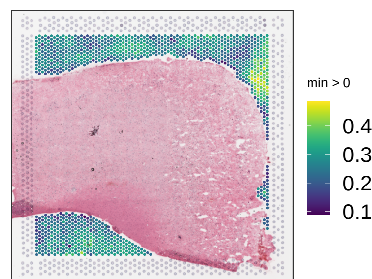
Br5415 expr_chrM_ratio
