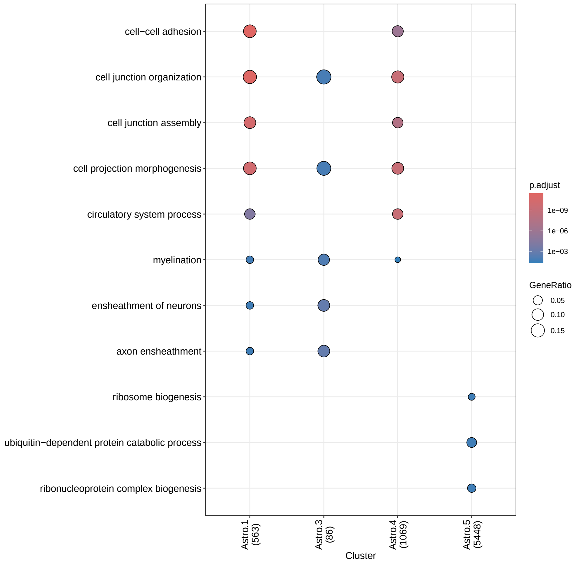
GO Enrichment: BP
