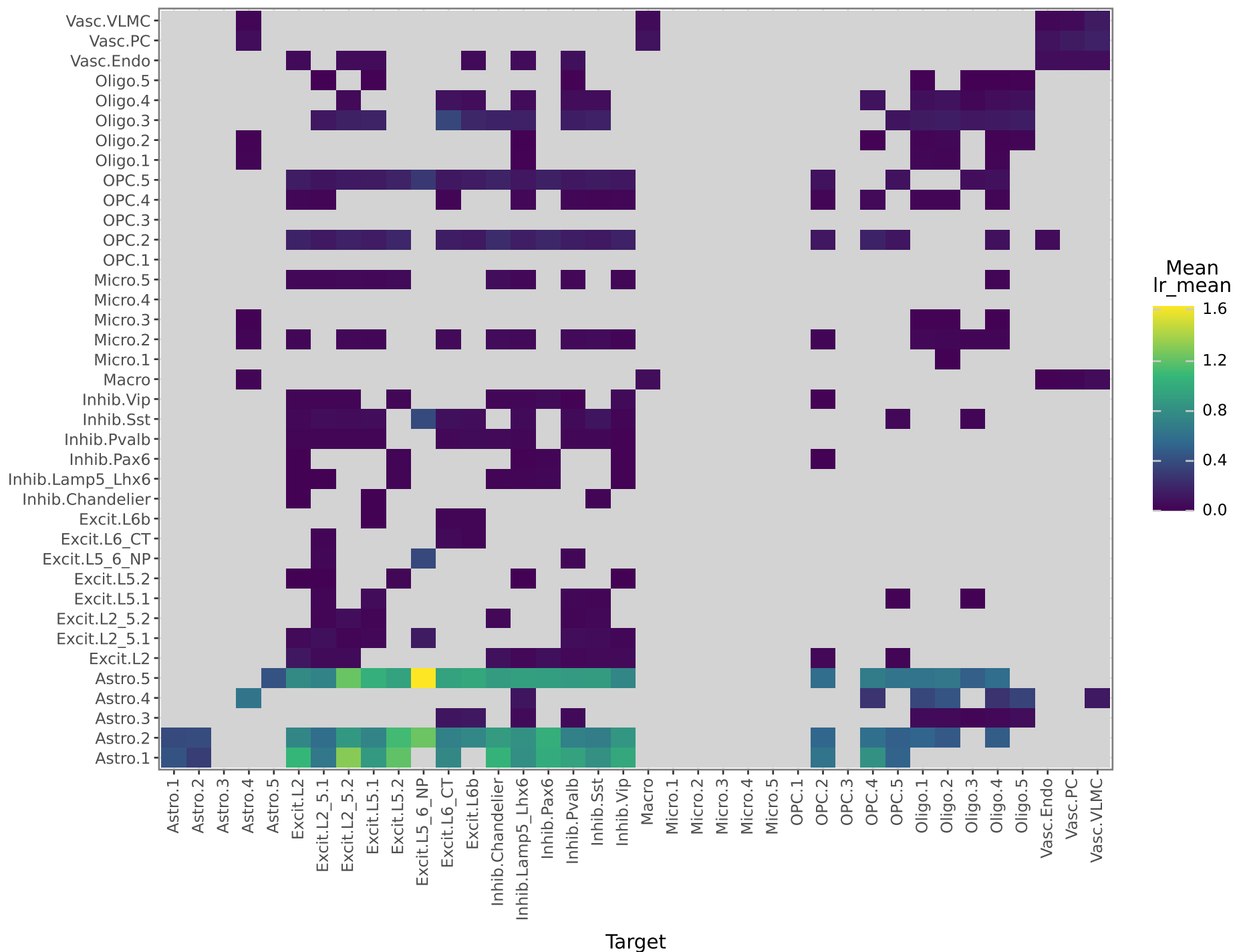
SPON1→APP: mean lr_mean (significant in \geq 4 samples)
