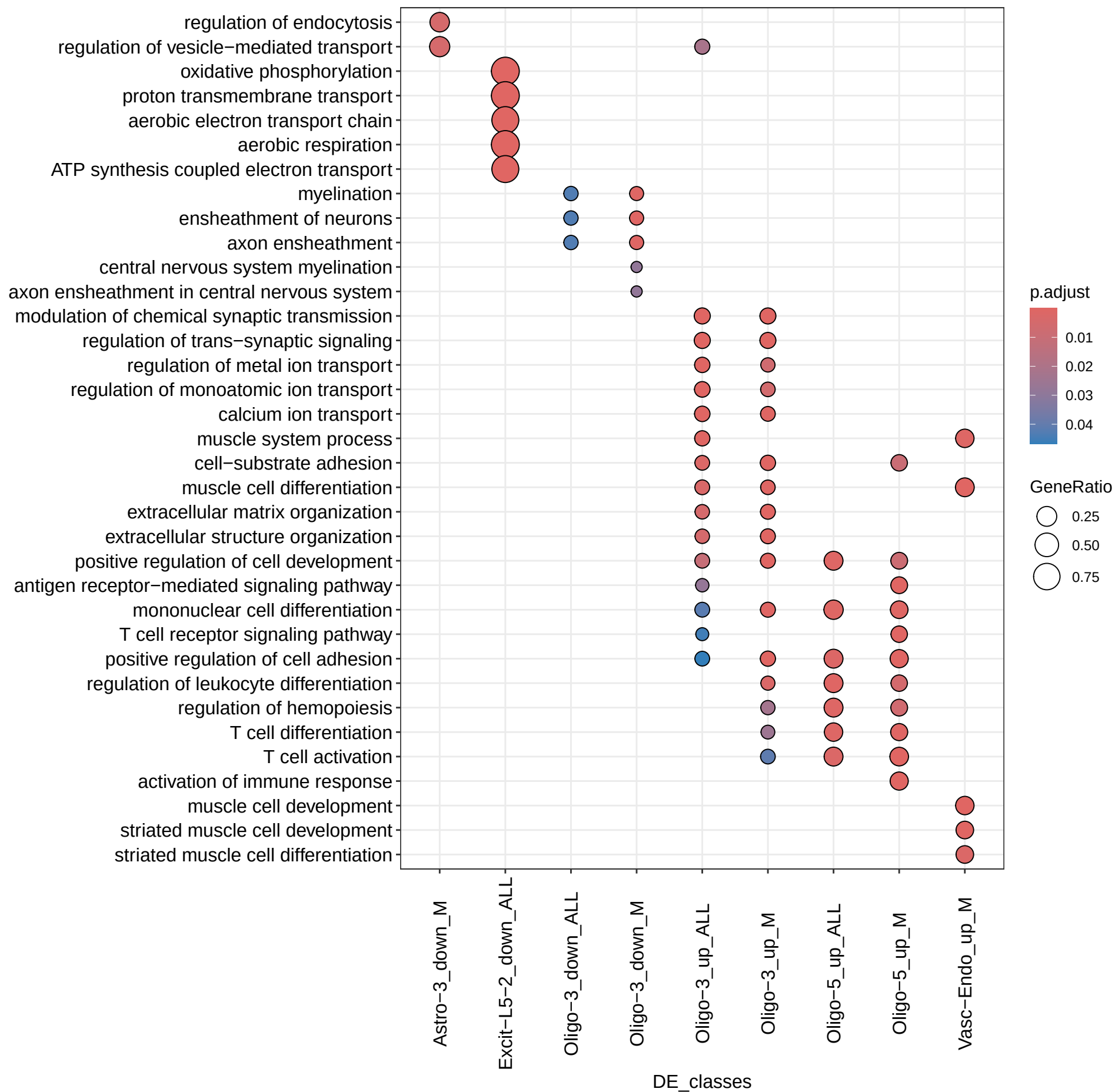
GO Enrichment: BP 2+ genes
