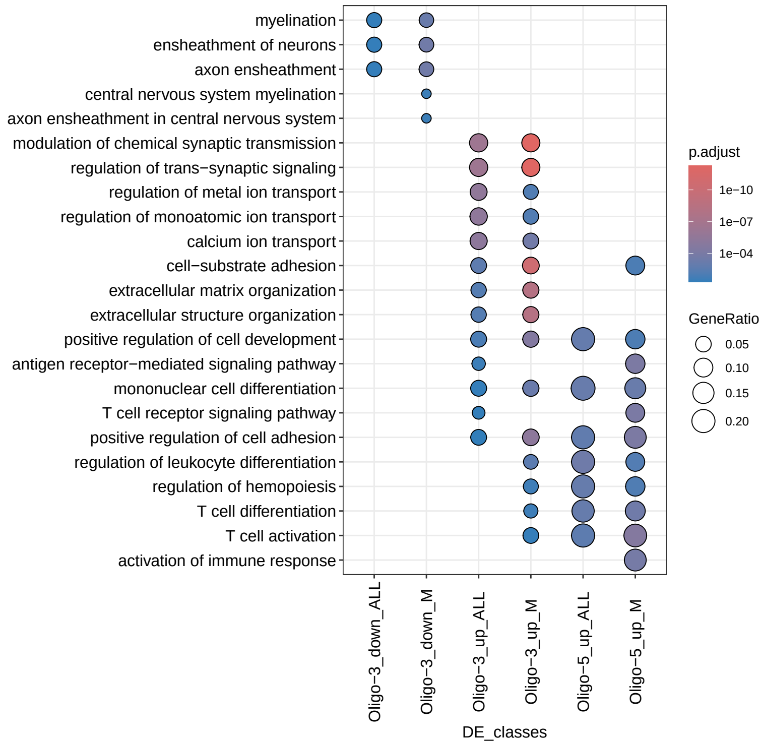
GO Enrichment: BP – Oligo, 5+ genes
