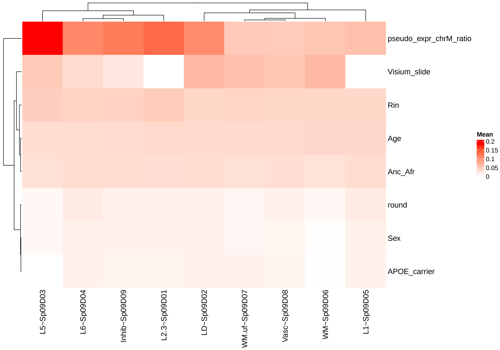
Visium VarPart – carrier
