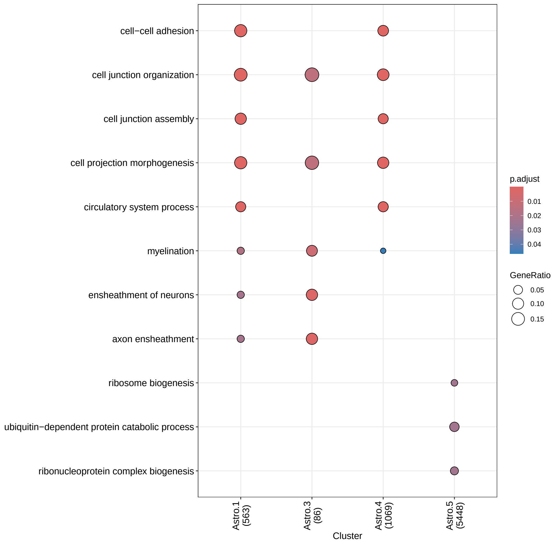
GO Enrichment: BP
