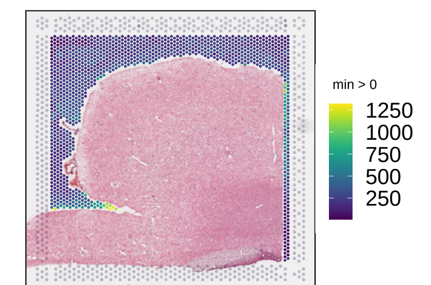
V13Y24-340_A1 sum_gene
