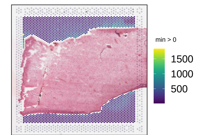
V13Y24-343_C1 sum_gene
