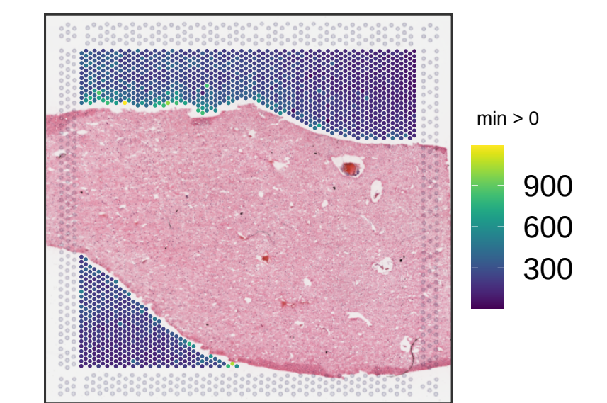
V13B23-363_C1 sum_gene
