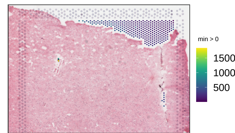
V13Y24-343_A1 sum_gene
