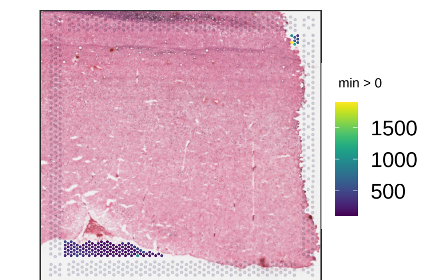
V13B23-363_A1 sum_gene
