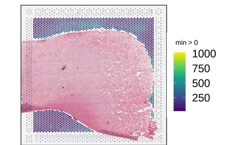
V13Y24-344_B1 sum_gene
