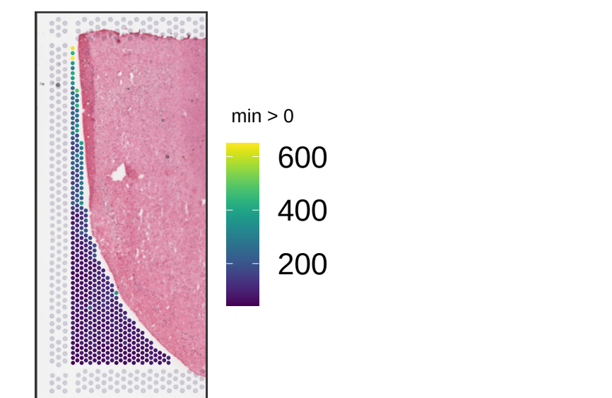
V13B23-365_D1 sum_gene
