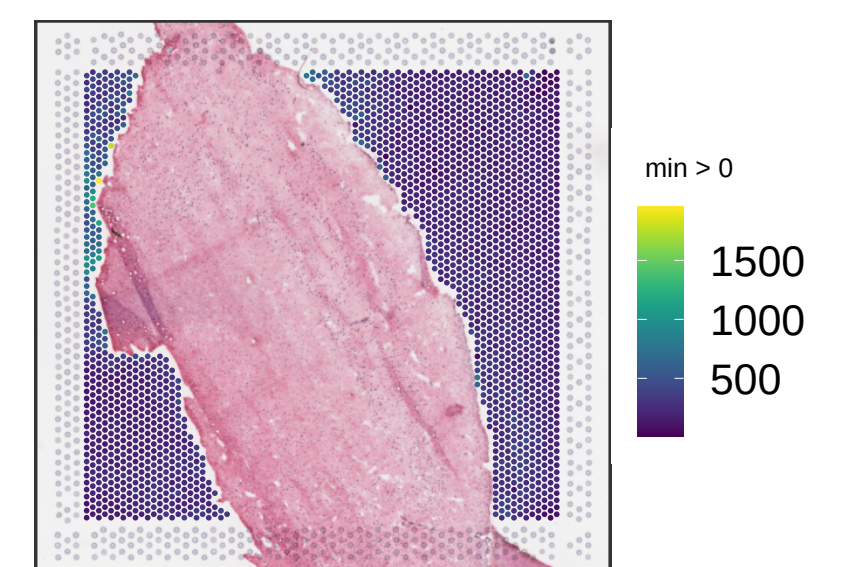
V13Y24-340_B1 sum_gene
