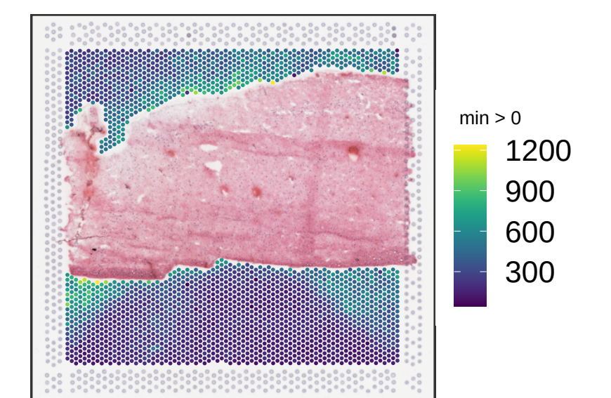
V13Y24-340_D1 sum_gene
