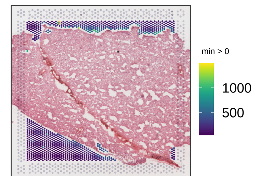
V13Y24-344_D1 sum_gene
