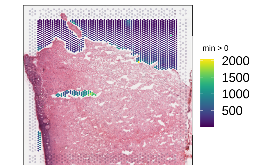
V13Y24-342_C1 sum_gene
