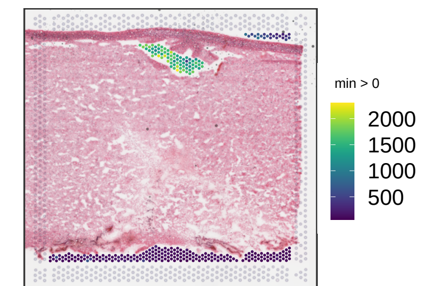
V13B23-365_C1 sum_gene
