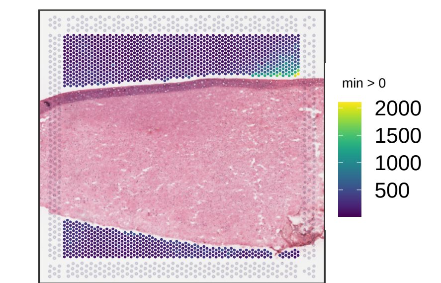
V13B23-364_C1 sum_gene
