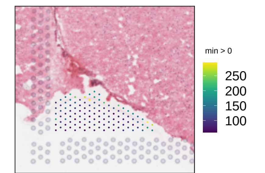
V13B23-364_B1 sum_gene
