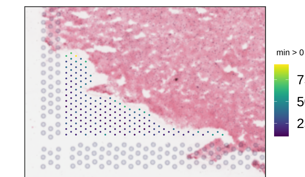
V13B23-363_B1 sum_gene
