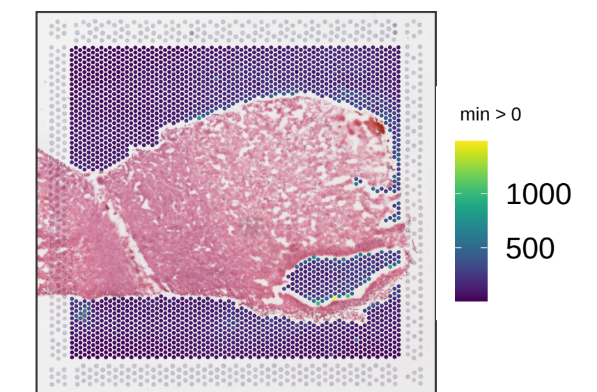
V13Y24-344_C1 sum_gene
