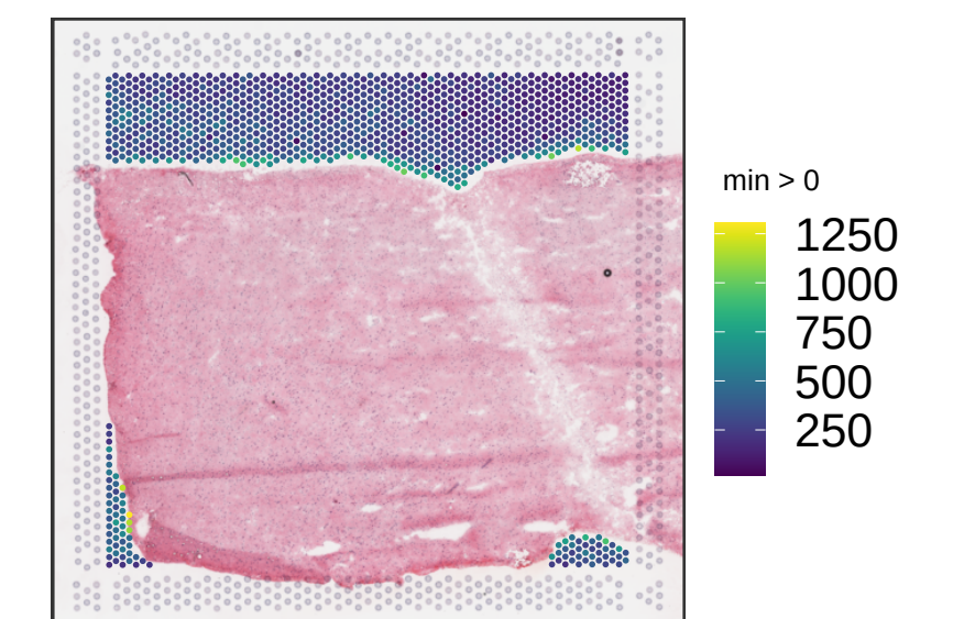
V13Y24-342_A1 sum_gene
