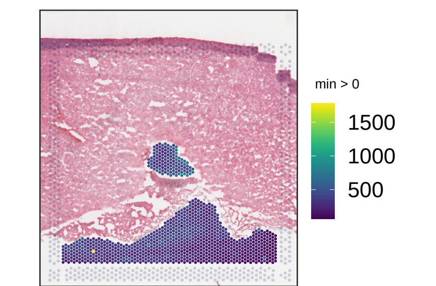
V13B23-364_A1 sum_gene
