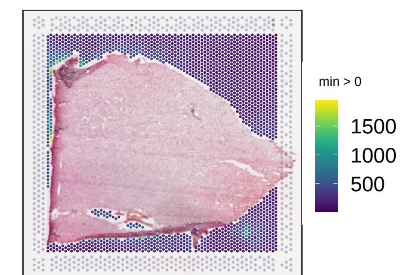
V13Y24-340_C1 sum_gene
