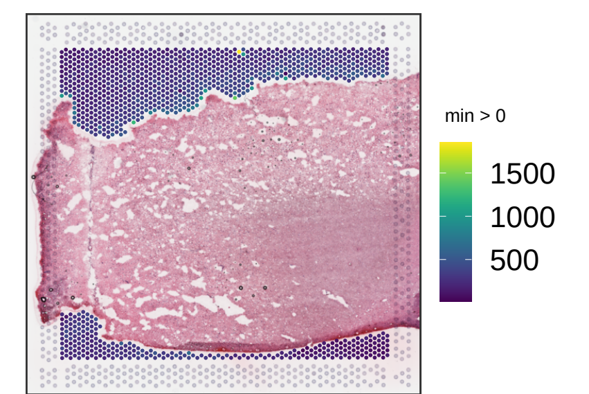
V13Y24-343_B1 sum_gene
