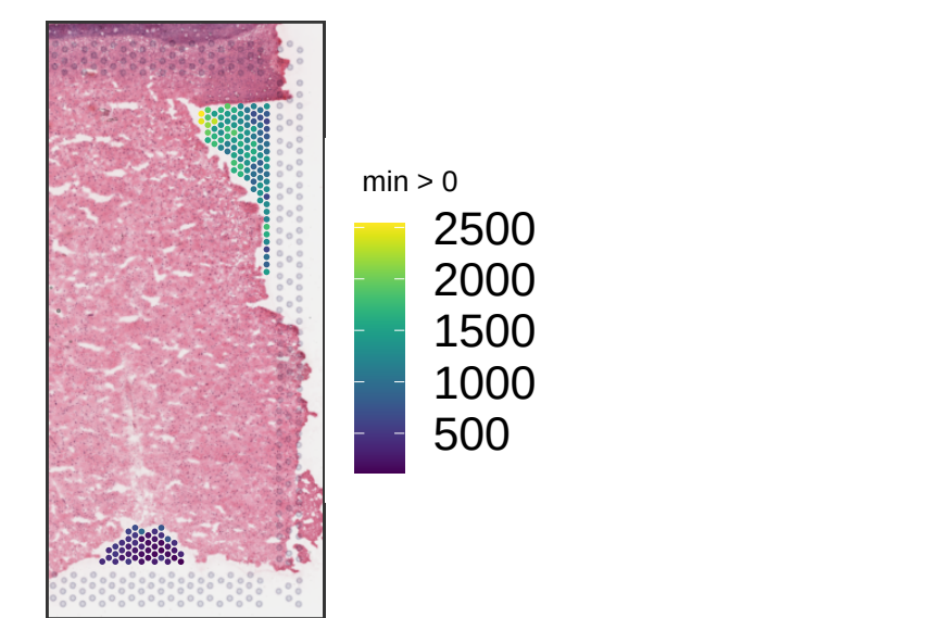
V13B23-363_D1 sum_gene
