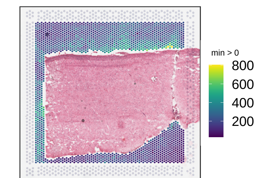
V13B23-366_D1 sum_gene
