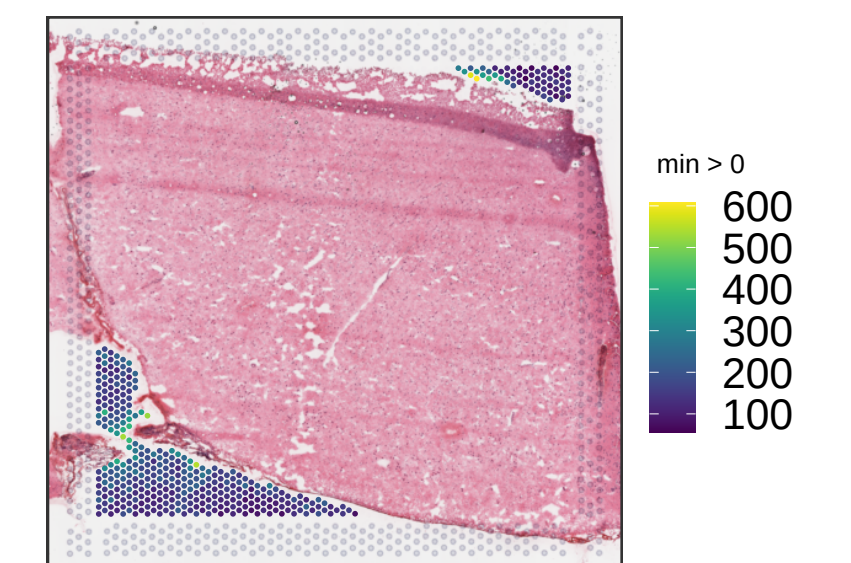
V13B23-365_B1 sum_gene
