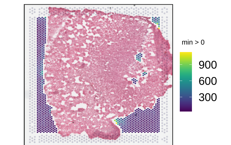
V13B23-366_C1 sum_gene
