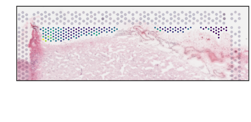
V13Y24-342_B1 sum_gene
