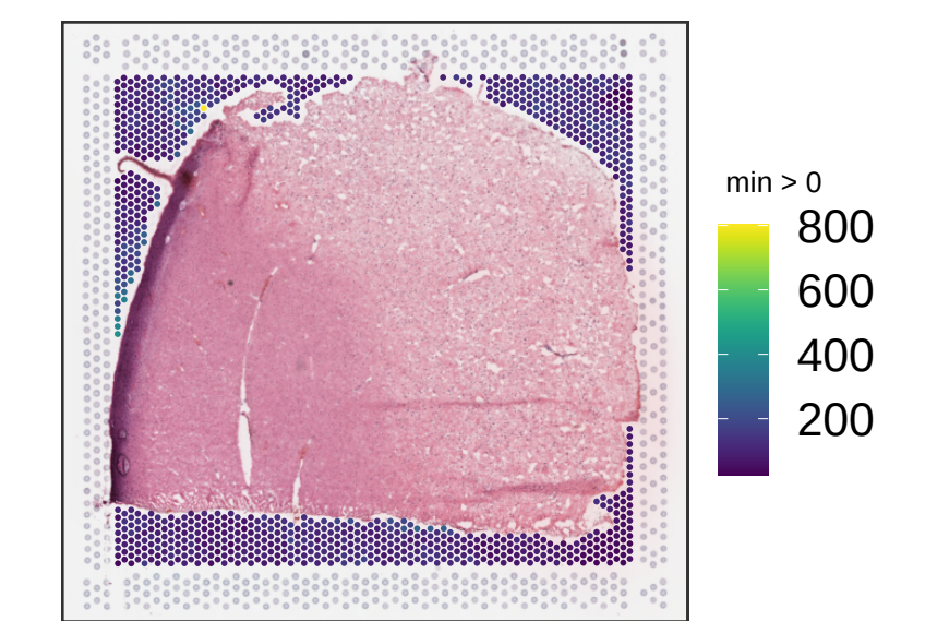
V13Y24-343_D1 sum_gene
