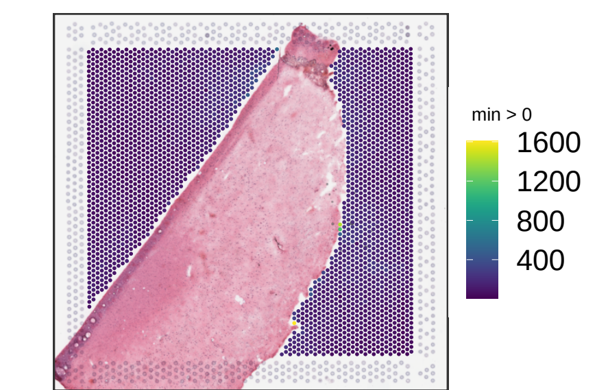
V13Y24-344_A1 sum_gene
