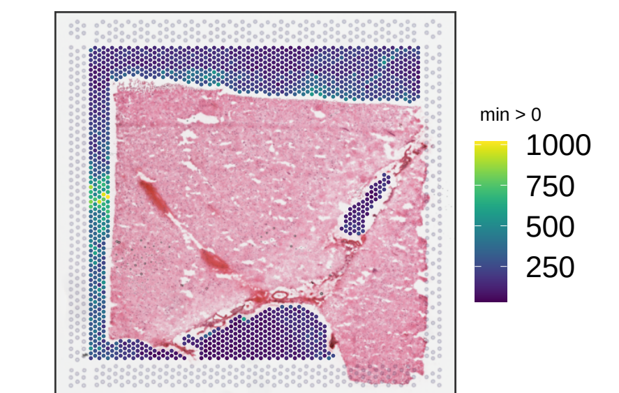
V13B23-366_B1 sum_gene
