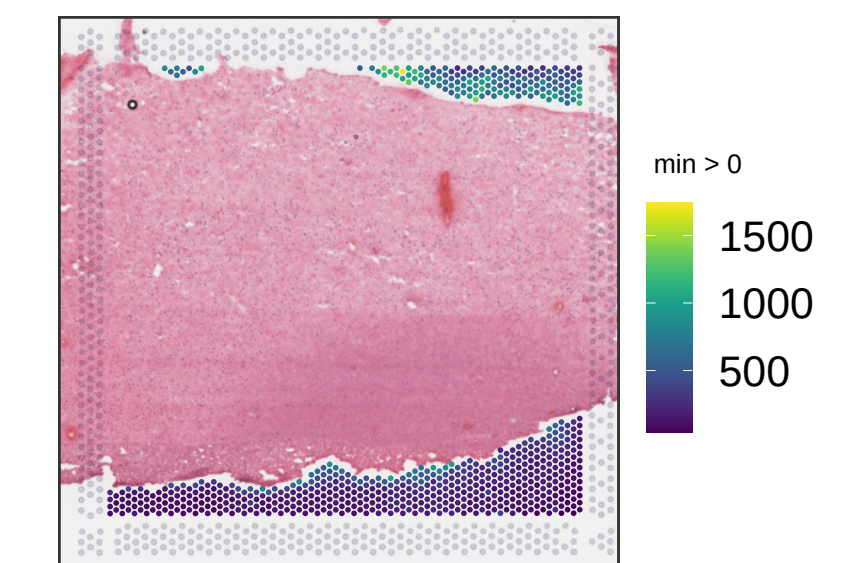
V13B23-365_A1 sum_gene
