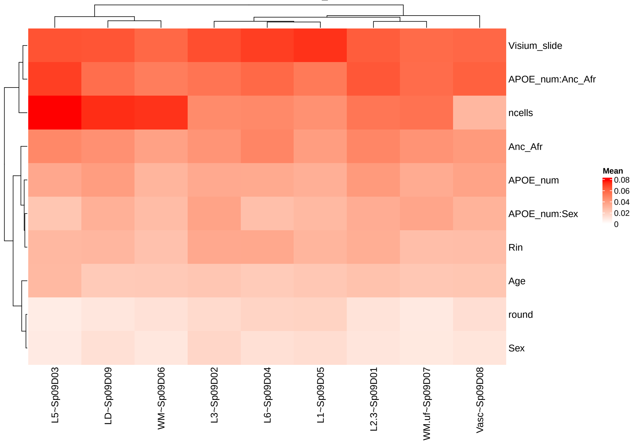
Visium VarPart – numeric_i
