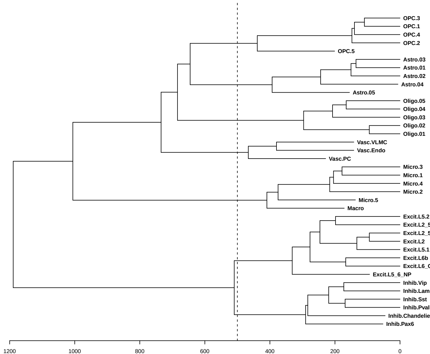
hierarchical cluster dend
